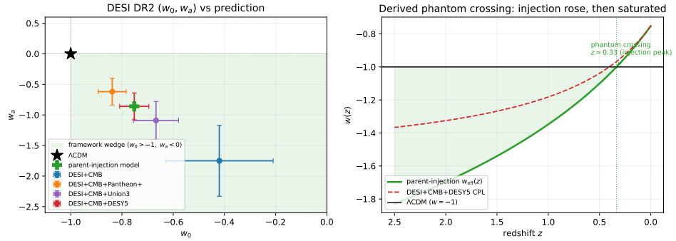
Figure 6.2: Dark energy as parent accretion vs DESI DR2. Left: the four DESI DR2 (w_0, w_a) fits all fall in the framework’s wedge ( w_0 > -1, w_a < 0 , shaded); \Lambda CDM (star) sits at its corner, disfavoured at 2.8\text{--}4.2\sigma . Right: the peaked-injection w_{\text{eff}}(z) of (6.1) crosses w = -1 at the injection peak z_{\text{cross}} \approx 0.33 (shaded: phantom epoch), tracking the DESI CPL reconstruction through the constrained range. Values flagged for verification against the published tables.
