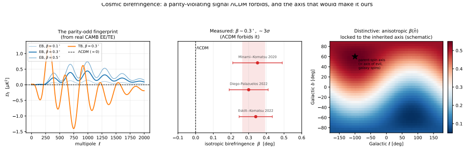
Figure 7.1: Cosmic birefringence as an Eternal Dawn signature. Left : the parity-odd EB and TB spectra a rotation \beta produces, computed from the real CAMB EE/TE transfer via (7.1); \Lambda CDM predicts them identically zero (dashed). Middle : the measured isotropic \beta \simeq 0.3^\circ (Planck, Planck+WMAP) against the \Lambda CDM zero it excludes. Right : the distinctive, uniquely-ED component—an anisotropic \beta(\hat{n}) locked to the inherited spin axis, predicted to coincide with the axis of evil / galaxy-spin axis (shown as a shape; the amplitude is not derived). Reproducible as figures/scripts/ch07_birefringence.py.
