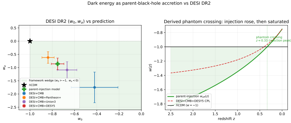
Figure 6.5: Dark energy as parent accretion versus DESI. Left : every DESI ( w_0, w_a ) combination sits in the framework’s predicted wedge ( w_0 > -1 , w_a < 0 ), where the parent-injection model also lands. Right : the derived w(z) —a phantom crossing produced by accretion that rose then saturated, not a free sign choice. Reproducible as figures/scripts/ch06_desi.py .
