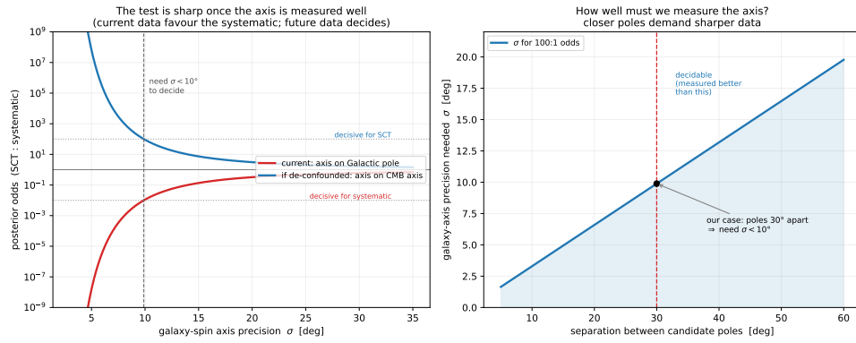
Figure 6.3: The shared-axis test as a precision question. Left : posterior odds (CMB axis:Galactic pole) versus the precision \sigma of the galaxy-spin axis; today’s geometry (axis on the Galactic pole) favours the systematic, a de-confounded axis on the CMB axis would favour the framework, and either way \sigma \lesssim 10^\circ is needed. Right : the candidate poles are \sim 30^\circ apart, setting the \sim 10^\circ precision target. Reproducible as figures/scripts/ch08_shared_axis.py .
