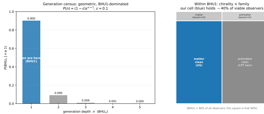
Figure 6.4: The supravarse census of viable observers. Left : the generation tower is geometric and first-generation-dominated; we are in the n = 1 bar. Right : within that generation, our cell (matter, clean family) holds \sim 40\% of viable observers, with an identical antimatter CPT twin. Our footprint is the typical, dominant cell. Reproducible as figures/scripts/ch08_census.py .
