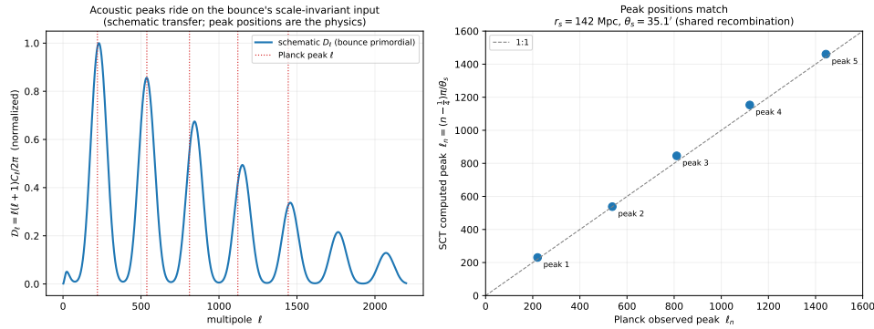
Figure 8.4: The acoustic peaks. The bounce’s scale-invariant primordial input, carried through the standard post-bounce plasma, yields a sound horizon r_s \simeq 142 Mpc and a peak series matching the observed Planck multipoles to a few percent. The peak heights are computed in Figure 8.5. Reproducible as figures/scripts/ch09_acoustic.py.
