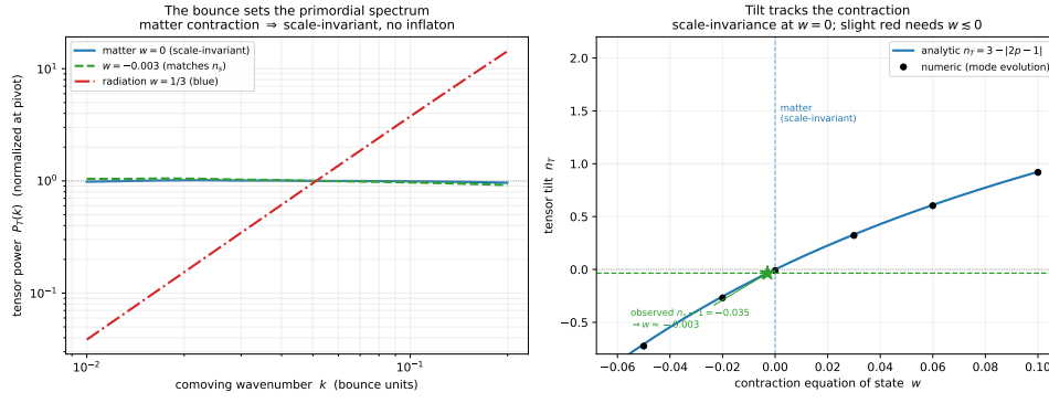
Figure 8.3: The primordial spectrum from the Einstein–Cartan bounce. Left: the tensor power spectrum is flat (scale-invariant) for a matter-dominated contraction and blue for radiation—scale invariance with no inflaton. Right: the tilt n_T versus contraction equation of state on the analytic curve; w = 0 is scale-invariant, and the observed tilt corresponds to w \approx -0.003 . Reproducible as figures/scripts/ch09_primordial.py.
