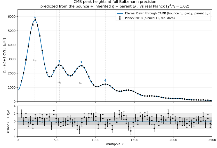
Figure 8.5: The peak heights , at full Boltzmann precision, against the real Planck 2018 binned TT spectrum. The standard recombination transfer (CAMB), fed an Eternal Dawn parameter set whose values are sourced — n_s from the bounce, \omega_b from the inherited \eta , \omega_c from the parent’s projected mass—reproduces the measured spectrum at \chi^2/N \simeq 1.0 over 83 band powers (residuals, lower panel, scatter within \pm 2\sigma ). The first peak’s height fixes the baryon density (the odd/even ratio D_1/D_2 \simeq 2.2 ), the third peak the dark-matter density ( D_1/D_3 \simeq 2.3 ); \omega_c/\omega_b \simeq 5.4 is the baryon fraction f \approx 1/6 the membrane filter explains as natural (§8.5). Reproducible as figures/scripts/ch09_peak_heights.py.
