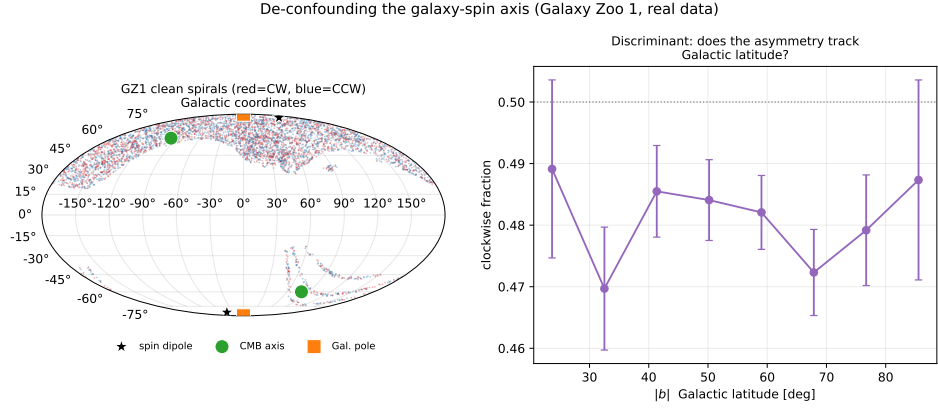
Figure 6.1: De-confounding the galaxy-spin axis on Galaxy Zoo 1 (clean spirals). Left : the SDSS northern footprint (red clockwise, blue counter); the fitted spin dipole (star) sits on the Galactic pole, 35^\circ from the CMB axis. Right : the clockwise fraction sits a few percent below 0.5 independent of Galactic latitude—a global perception offset, not a significant dipole (shuffle null p = 0.62 ). Reproducible as figures/scripts/ch08_galaxy_dipole.py .
