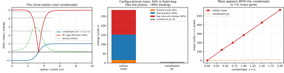
Figure 6.3: Configurational mass. From (6.6) the torsiton mass is dominantly condensate field energy and is proportional to the symmetry-breaking amplitude v = f_\pi : turn off the condensate and the mass vanishes. Mass is a property of the bound configuration, not an intrinsic tag.
