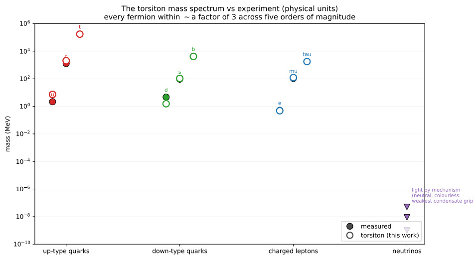
Figure 9.2: The torsiton mass spectrum versus experiment, in physical units. Open circles: the torsiton masses of Eq. (9.1); filled: the measured values; coloured by family. Every one of the twelve fermions lands within about a factor of three of its measured mass across five orders of magnitude—the charged leptons within 10–20%—and the neutrinos sit at the floor, forced light by their vanishing handle. The relative placement is qualitatively exact; the absolute values are within an order of magnitude.
