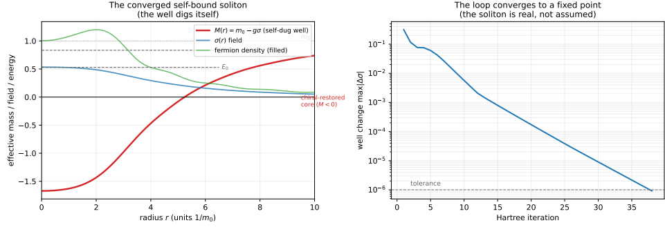
Figure 6.2: The self-consistent torsiton. The Hartree loop (levels \rightarrow density \rightarrow condensate \rightarrow well) of Section 6.3 converges to a self-bound profile M(r) = m - g\sigma(r) with a discrete bound spectrum E_n . Reproducible from sims/src/cartasis_sims/self_consistent.py .
