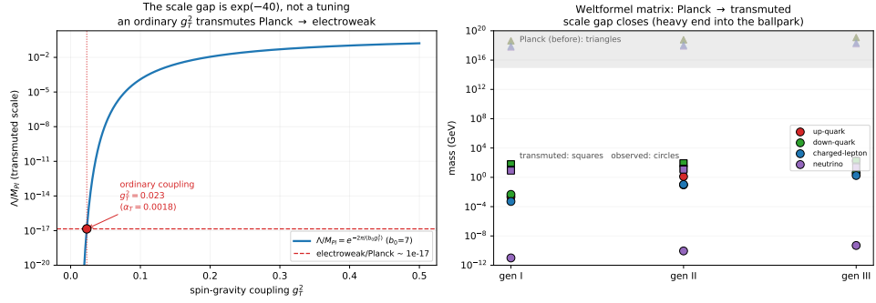
Figure 6.1: The infrared scale by dimensional transmutation, Eq. (6.1). The electroweak-to-Planck ratio is e^{-40} \approx 10^{-17} , the exponential of an ordinary coupling g^2 \sim 0.02 (weaker than electromagnetism). Fixing the scale here, once, lets the rest of Part II work in physical units—the same step \Lambda_{\text{CDM}} makes for \Lambda_{\text{QCD}} .
