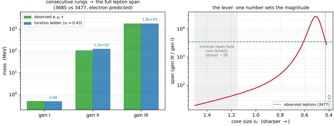
FIG. 1. The hierarchy as one number. Left : the consecutive radial ladder n = 1, 2, 3 against a core of a single sharpness s_T reproduces the whole charged-lepton span, with the electron’s tiny mass a prediction once the heaviest rung sets the scale. Right : the lever (Eq. 9)—the span sweeps orders of magnitude as the core sharpens; the observed spread is crossed at a sharp-but-physical core.
