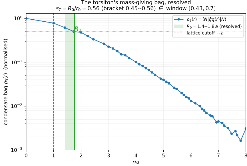
FIG. 3. The torsiton’s mass-giving bag, resolved. The connected three-body condensate \rho_3(r) = \langle N|\bar{q}q(r)|N\rangle on the dynamical ensemble ( t_{\text{snk}} = 20 ). The half-density radius R_0 lifts off the lattice cutoff ( R_0 = 1.4\text{--}1.8 a across sink times), giving s_T = R_0/r_0 inside the productive window [0.43, 0.70] .
