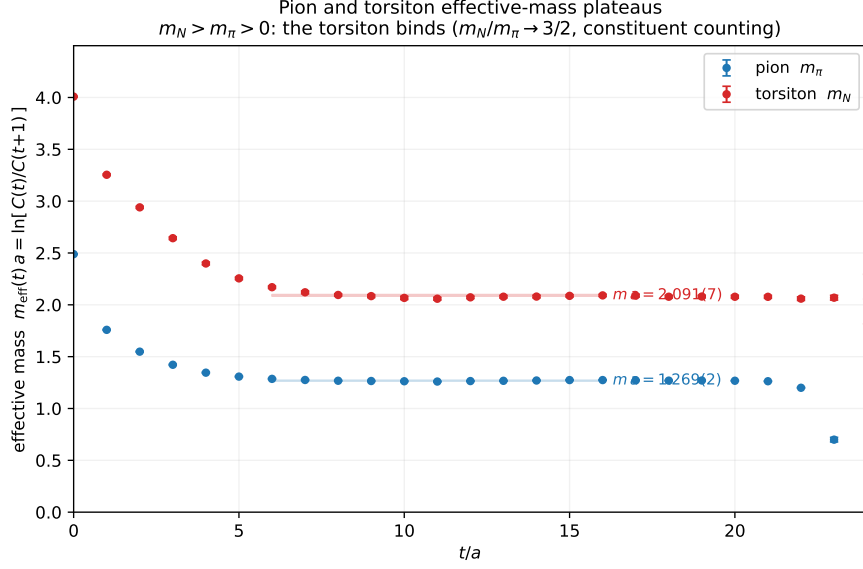
FIG. 2. The pion and torsiton (nucleon) effective-mass plateaus on the dynamical ensemble, m_{\text{eff}}(t) a = \ln[C(t)/C(t+1)] with jackknife errors over configurations and the plateau-fit bands. A clean plateau at m_N > m_\pi > 0 is the torsiton, bound non-perturbatively; the ratio approaches the constituent-counting value m_N/m_\pi \rightarrow 3/2 at heavy quark mass.
