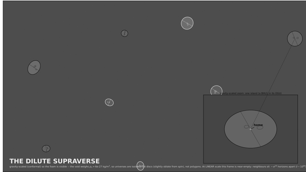
Figure 10.3: The dilute supraverse, gravity-scaled (sizes and spacings illustrative, not linear). The weighted void ( \rho_v \sim 6 \times 10^{-27} \text{ kg m}^{-3} , faintly speckled with zero-point energy) dominates; universes are sparse, round , isolated islands (gravity wells with chirality-toned Cartasis membranes, faint nested BHU children). The inset zooms one, marking home . At a literal linear scale the frame would be near-empty—neighbours lie \sim e^{I/4} horizons apart—so the void’s weight keeps the islands round while the dilution makes the true gaps astronomically larger than drawn.
