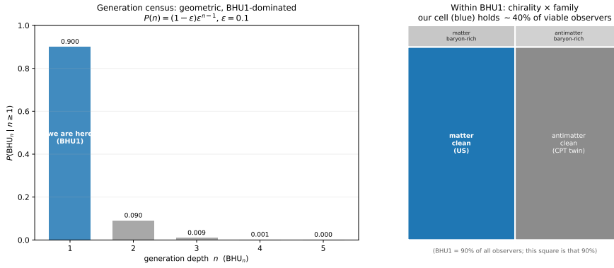
Figure 8.3: The supravarse census of viable observers. Left : the generation tower is geometric and BHU 1 -dominated; we are in the n = 1 bar. Right : within BHU 1 , the chirality × family breakdown—our cell (matter, clean; blue) holds ~40% of all viable observers, with an identical antimatter CPT twin. Our footprint is the typical, dominant cell.
