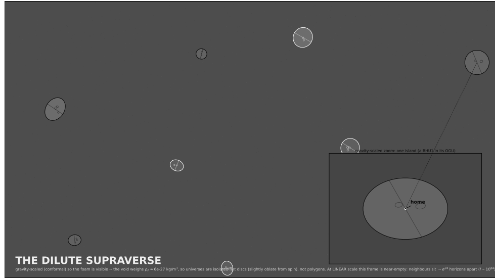
Figure 10.2: The dilute supraverse, gravity-scaled (sizes and spacings illustrative, not linear). The weighted void ( \rho_v \sim 6 \times 10^{-27} \text{ kg m}^{-3} , faintly speckled with zero-point energy) dominates; universes are sparse, round , isolated islands (gravity wells with chirality-toned Cartasis membranes, faint nested BHU children). The inset zooms one, marking home . At a literal linear scale the frame would be near-empty—neighbours lie \sim e^{1/4} horizons apart—so the void’s weight keeps the islands round while the dilution makes the true gaps astronomically larger than drawn.
