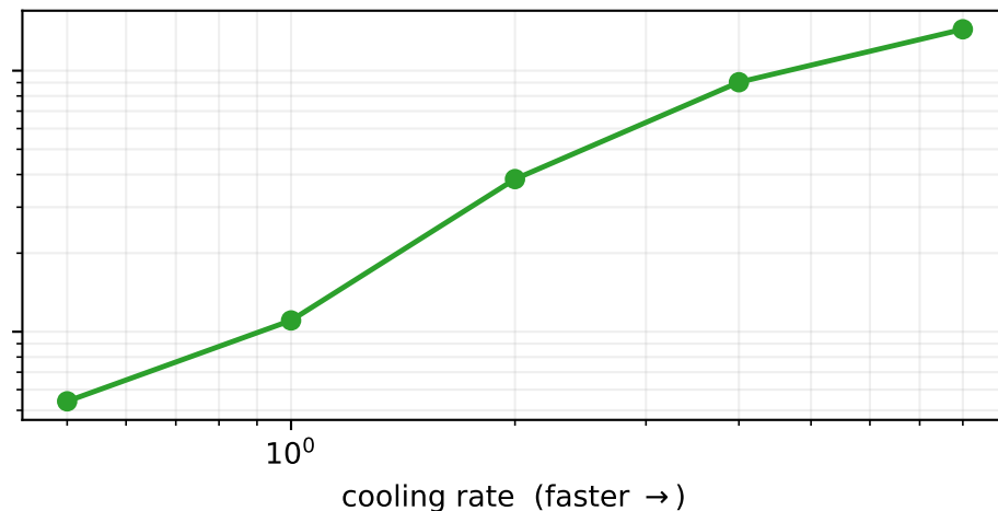
Kibble--Zurek: faster quench, more torsitons
