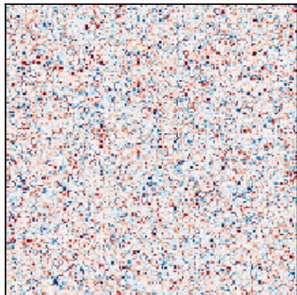
hot tally (disordered) T=0.83
