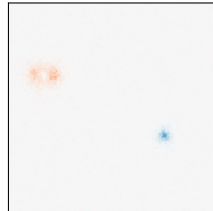
frozen relic (torsitons) T=0.00
