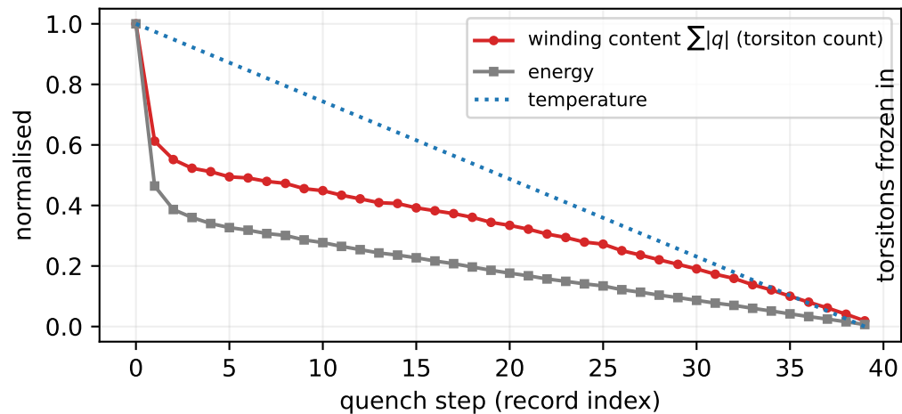
the fluid condenses: energy & winding fall, a relic set freezes
