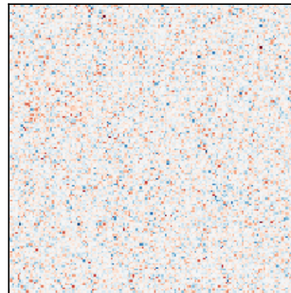
condensing (knots forming) T=0.35
