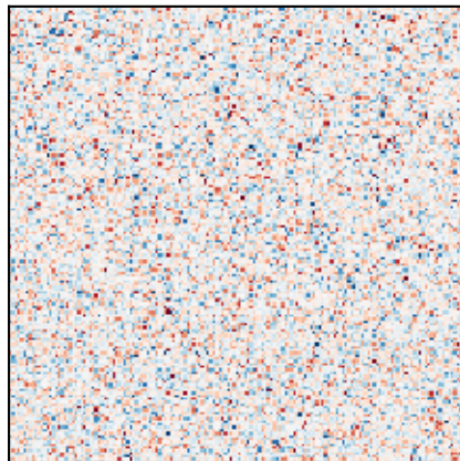
cooling (domains) T=0.62
