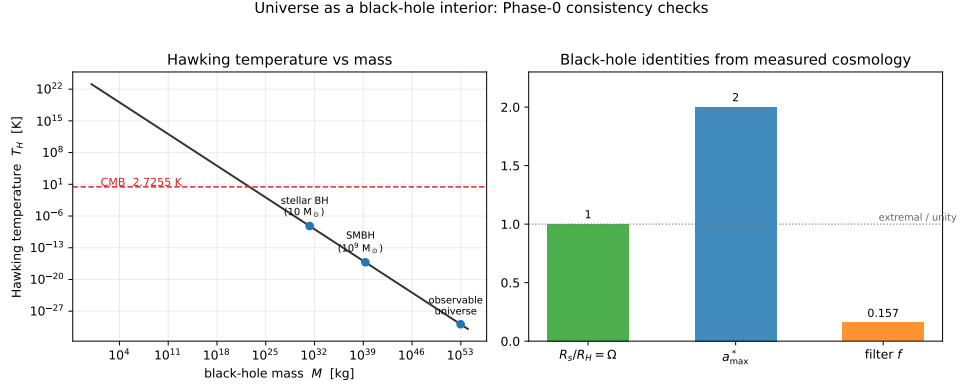
Figure 8.1: Phase-0 consistency checks, read straight off Planck cosmology. Left : the Hawking temperature T_H(M) puts the observable universe \sim 30 orders below the CMB, so the CMB is not present-horizon radiation. Right : the black-hole identities R_s/R_H = \Omega \approx 1 , maximal spin a_{\max}^* \approx 2 , and membrane filter f \approx 0.16 . Reproducible as figures/scripts/ch02_bh_first_light.py.
