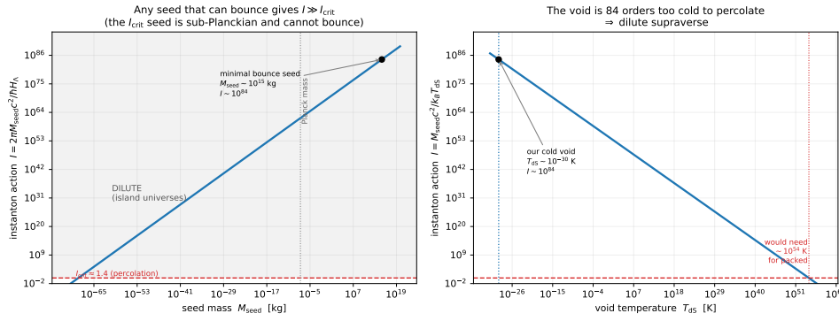
Figure 3.1: The OG-nucleation instanton action I = 2\pi M_{\text{seed}} c^2 / \hbar H_{\Lambda} (Equation (3.3)). Left: I versus seed mass; any seed massive enough to bounce ( \sim 10^{15} kg, the self-gravitating minimum) gives I \sim 10^{84} \gg I_{\text{crit}} \simeq 1.4 . Right: I versus void temperature; the cold de Sitter void ( \sim 10^{-30} K) is eighty-four orders too cold to percolate. The verdict is robust: a dilute, eternal-inflation-like supravse of isolated island universes. Reproducible as figures/scripts/ch05_instanton.py.
