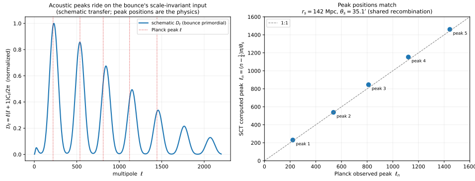
Figure 8.4: The acoustic peaks. The bounce’s scale-invariant primordial input, carried through the standard post-bounce plasma, yields a sound horizon r_s \simeq 142 Mpc and a peak series matching the observed Planck multipoles to a few percent. The peak heights await a full Boltzmann computation. Reproducible as figures/scripts/ch09_acoustic.py .
