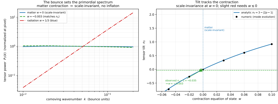
Figure 8.3: The primordial spectrum from the Einstein–Cartan bounce. Left: the tensor power spectrum is flat (scale-invariant) for a matter-dominated contraction and blue for radiation—scale invariance with no inflaton. Right: the tilt n_T versus contraction equation of state on the analytic curve; w = 0 is scale-invariant, and the observed tilt corresponds to w \approx -0.003 . Reproducible as figures/scripts/ch09_primordial.py .
