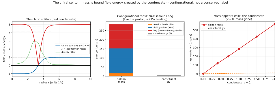
Figure 6.3: Configurational mass. From (6.6) the torsiton mass is dominantly condensate field energy and is proportional to the symmetry-breaking amplitude v = f_\pi : turn off the condensate and the mass vanishes. Mass is a property of the bound configuration, not an intrinsic tag.
