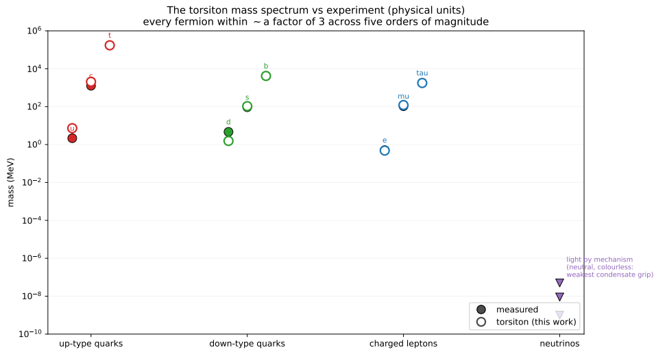
Figure 9.3: The per-tower-anchored comparison (three extra inputs beyond the single global scale of Figure 9.2): each tower’s overall normalisation fixed to one mass, the generations then predicted. Every charged fermion falls within a factor of three, the leptons within 10–20%—the geometric relationships are tight; only the inter-tower normalisations are owed.
