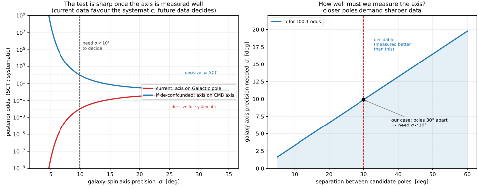
Figure 10.3: The shared-axis test as a precision question. Left : posterior odds (CMB axis:Galactic pole) versus the precision \sigma of the galaxy-spin axis; today’s geometry (axis on the Galactic pole) favours the systematic, a de-confounded axis on the CMB axis would favour the framework, and either way \sigma \lesssim 10^\circ is needed. Right : the candidate poles are \sim 30^\circ apart, setting the \sim 10^\circ precision target. Reproducible as figures/scripts/ch08_shared_axis.py.
