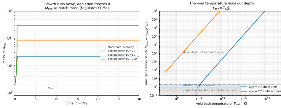
Figure 5.5: Left: growth trajectories from (5.6). In a static bath the hole runs away (finite-time blow-up); depleting a finite local patch freezes it at M_{\text{final}} \sim the patch mass—the regulator that keeps universe-holes finite. Right: the maximum generation depth D_{\text{max}} = T_{\text{supra}}/\tau_{\text{gen}} versus the void bath temperature ( \tau_{\text{gen}} \propto T_{\text{bath}}^{-3} ), for two supraversion ages. Below the sterile line no BHU forms (excluded by our existence); a narrow band gives the forced-shallow BHU 1-2 ; above it the depth is large and set by the branching ratio.
