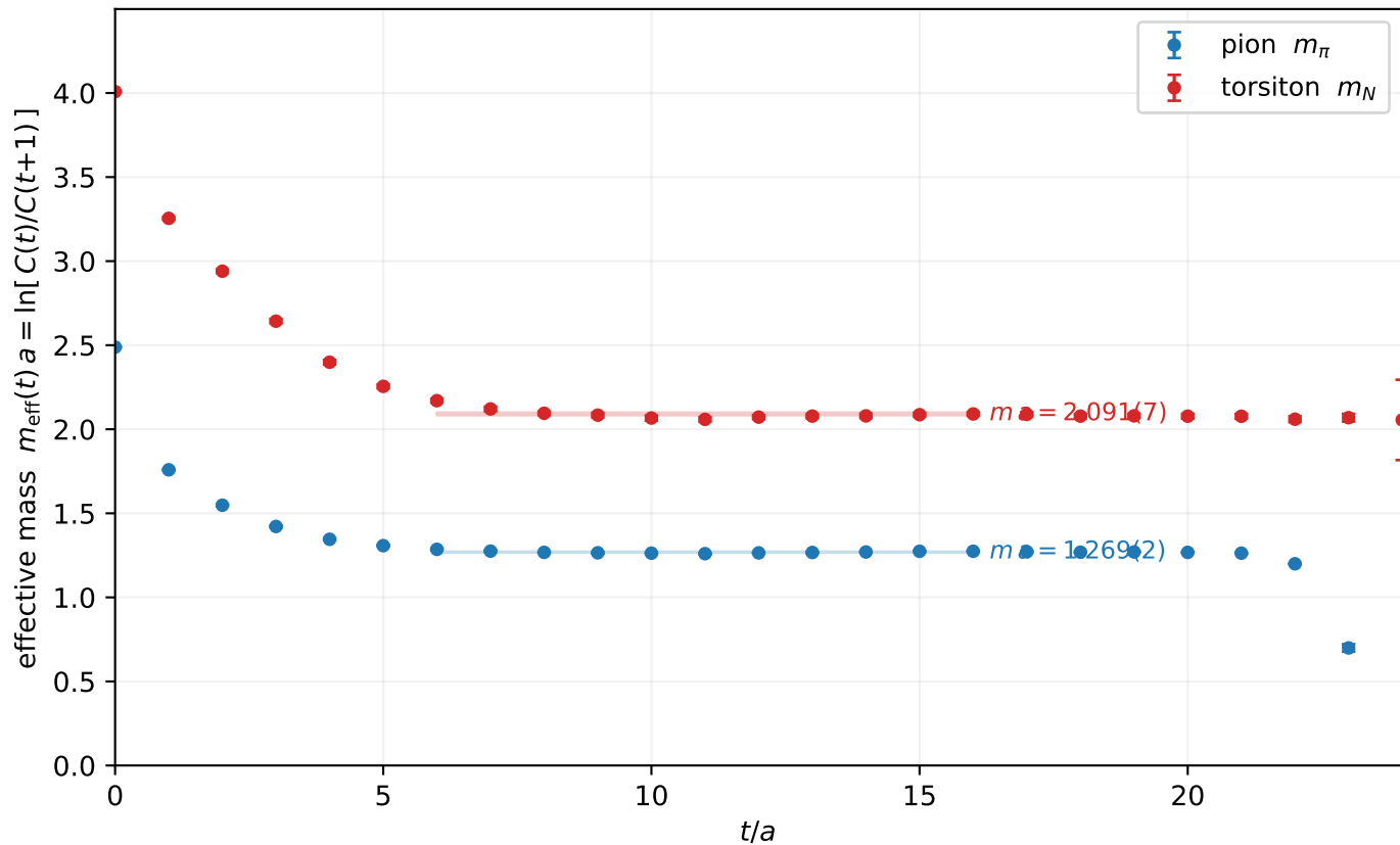
Pion and torsiton effective-mass plateaus m_N > m_\pi > 0 : the torsiton binds ( m_N/m_\pi \rightarrow 3/2 , constituent counting)
