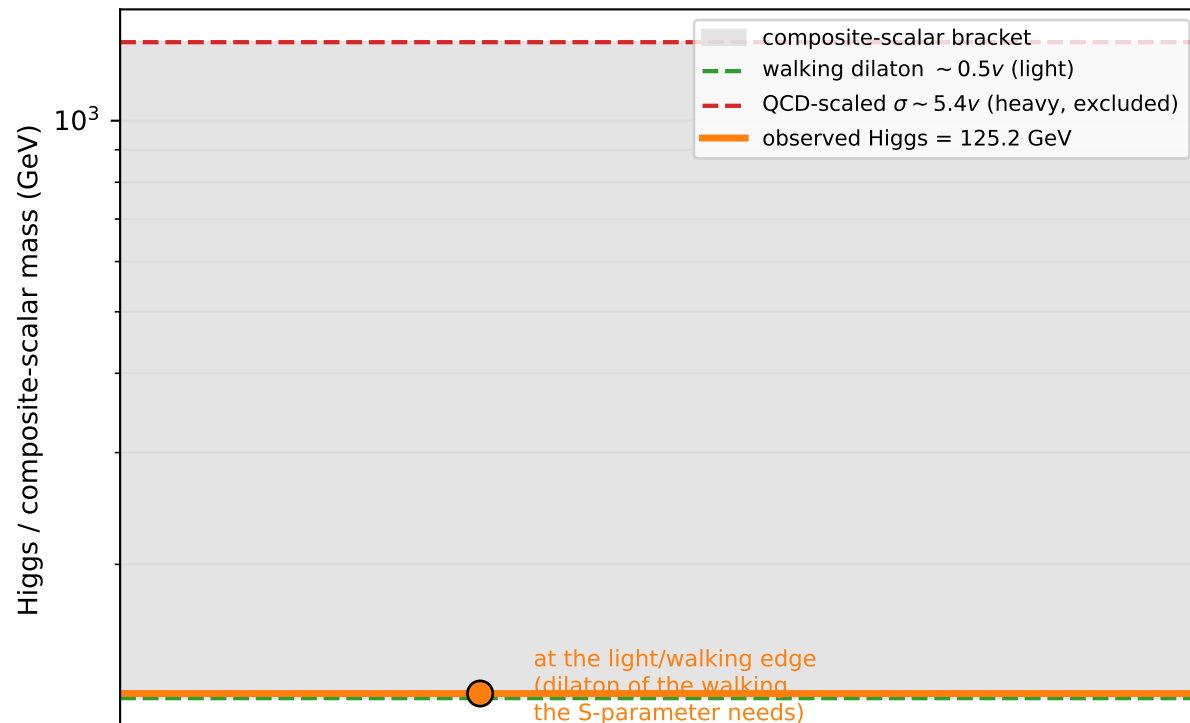
The Higgs as a composite scalar (bracketed) observed sits at the light edge -> walking
