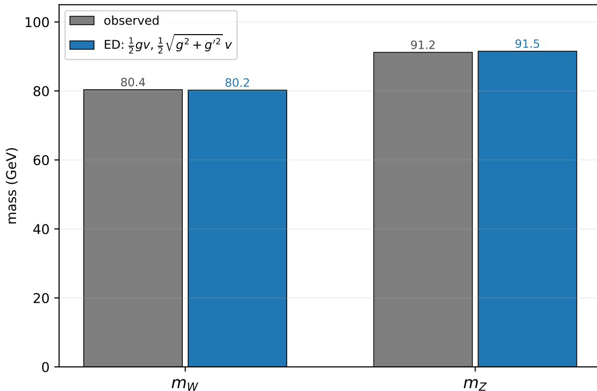
W, Z from the condensate scale (within 0.4%) custodial \rho = 1 : m_W = m_Z \cos \theta_W
