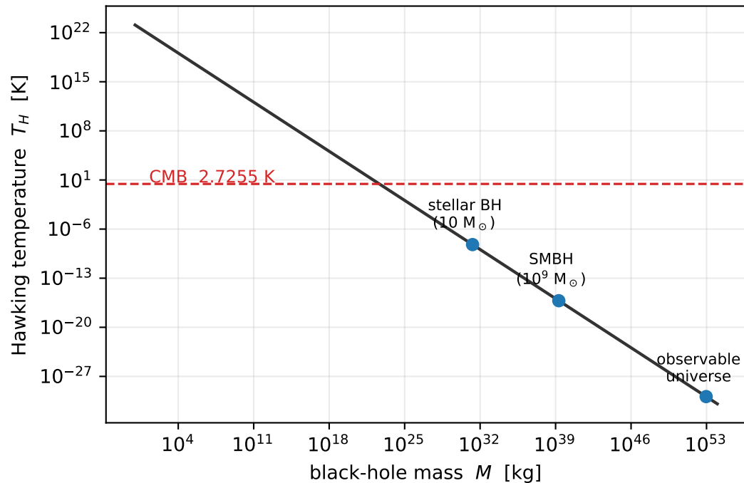
Hawking temperature vs mass
