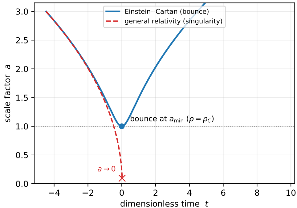
Collapse: bounce vs singularity
