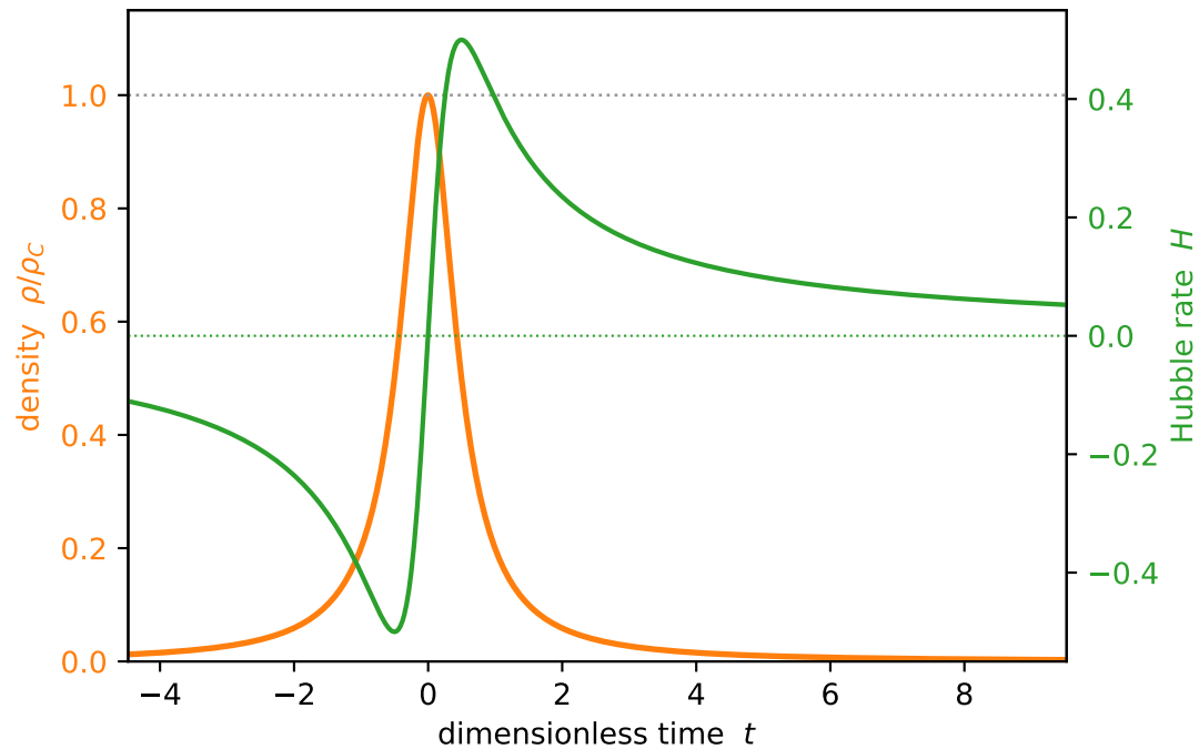
Density saturates at \rho_C , H crosses zero
