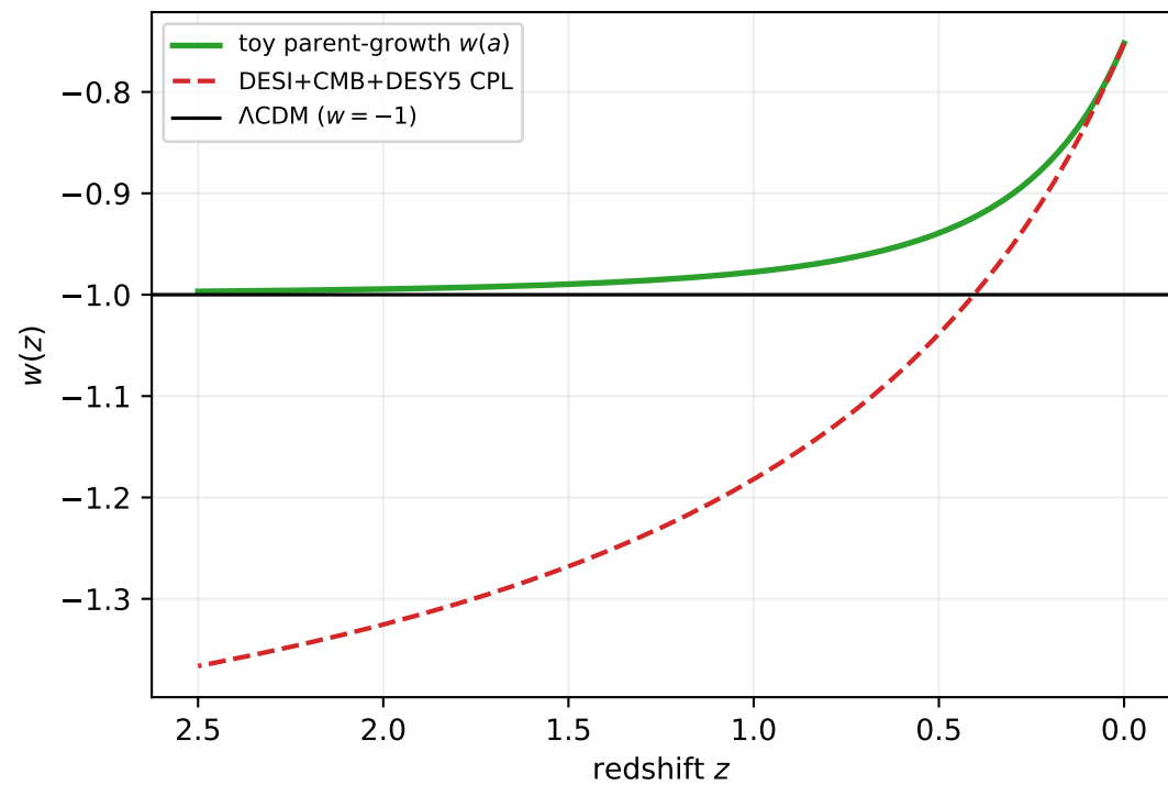
Toy matches ( w_0, w_a ) today; CPL goes phantom in the past
