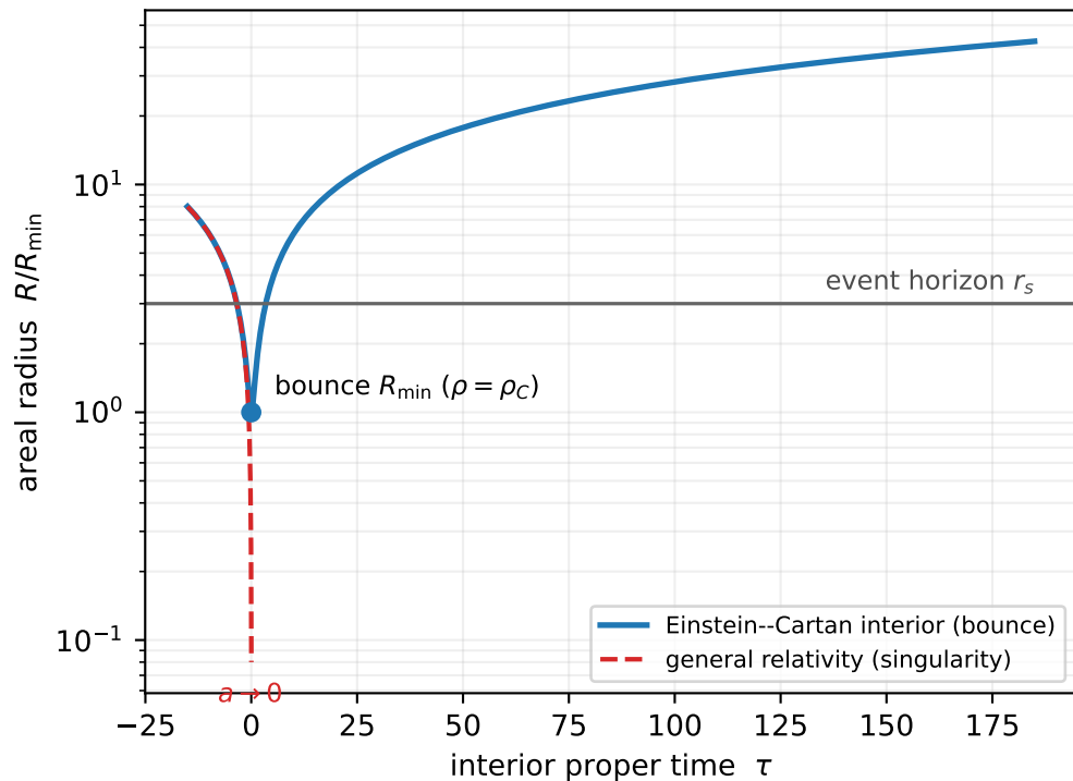
Interior: bounce hidden behind the horizon
