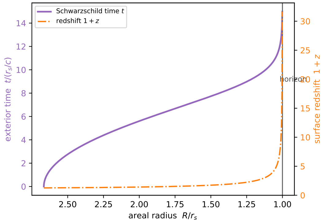
Exterior: surface freezes, light reddens to black
