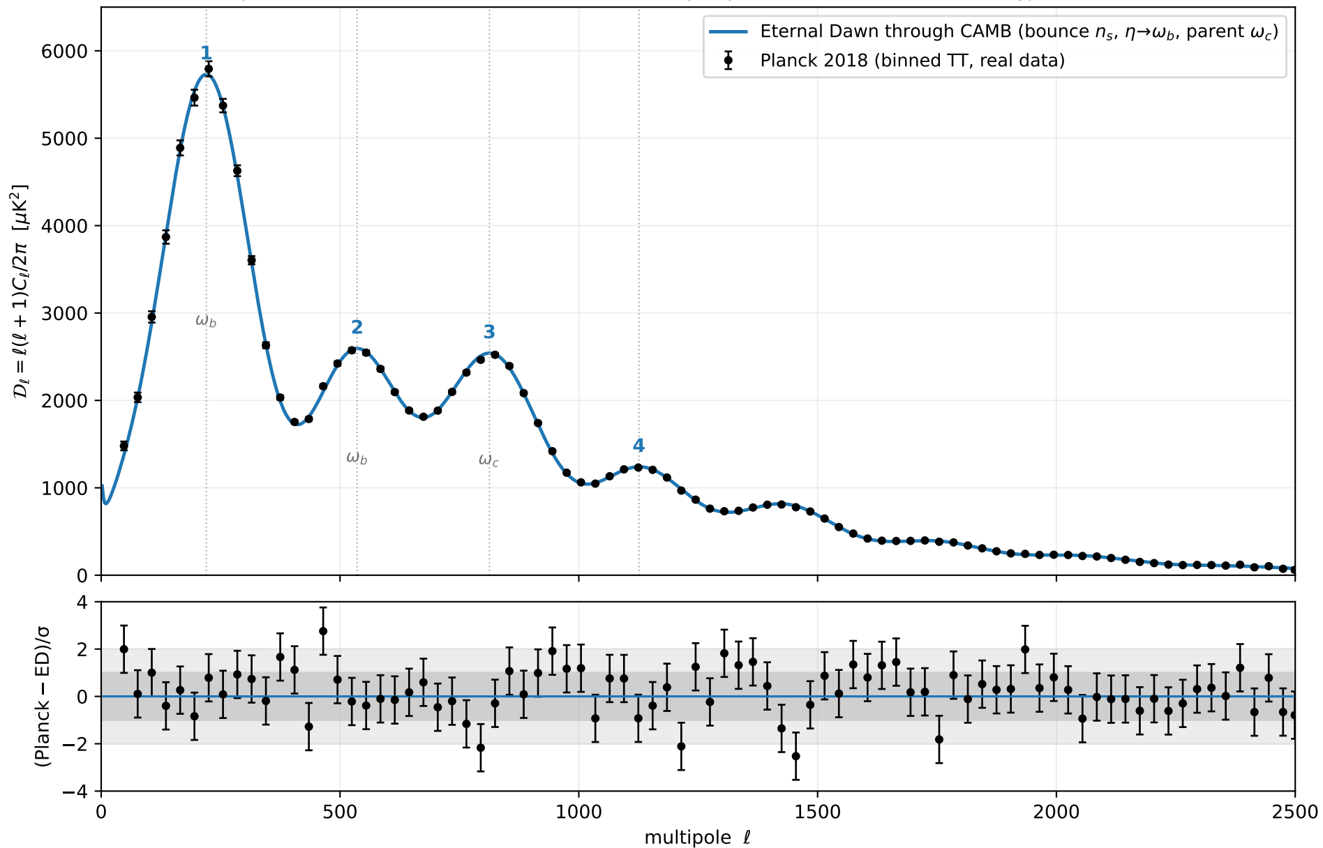
CMB peak heights at full Boltzmann precision predicted from the bounce + inherited \eta + parent \omega_c , vs real Planck ( \chi^2/N = 1.02 )
