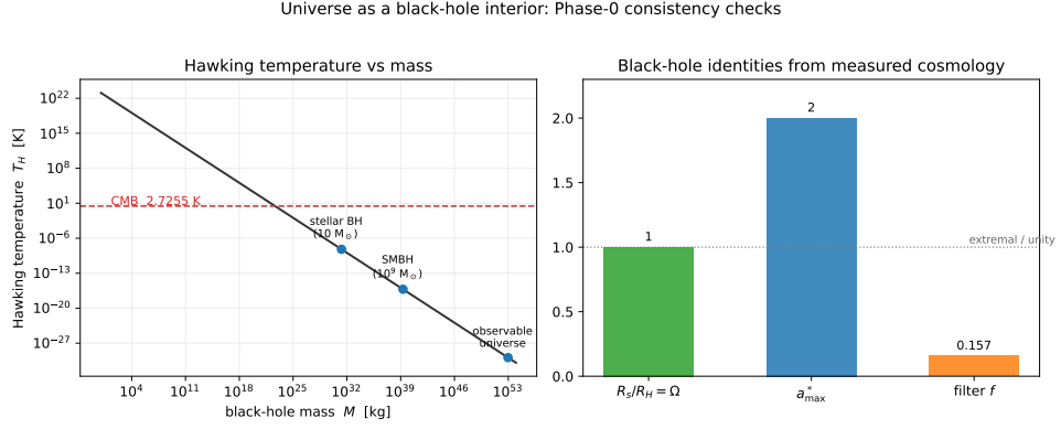
Figure 8.1: Phase-0 consistency checks, read straight off Planck cosmology. Left: the Hawking temperature T_H(M) puts the observable universe \sim 30 orders below the CMB, so the CMB is not present-horizon radiation. Right: the black-hole identities R_s/R_H = \Omega \approx 1 , maximal spin a_{\max}^* \approx 2 , and membrane filter f \approx 0.16 . Reproducible as figures/scripts/ch02_bh_first_light.py.
