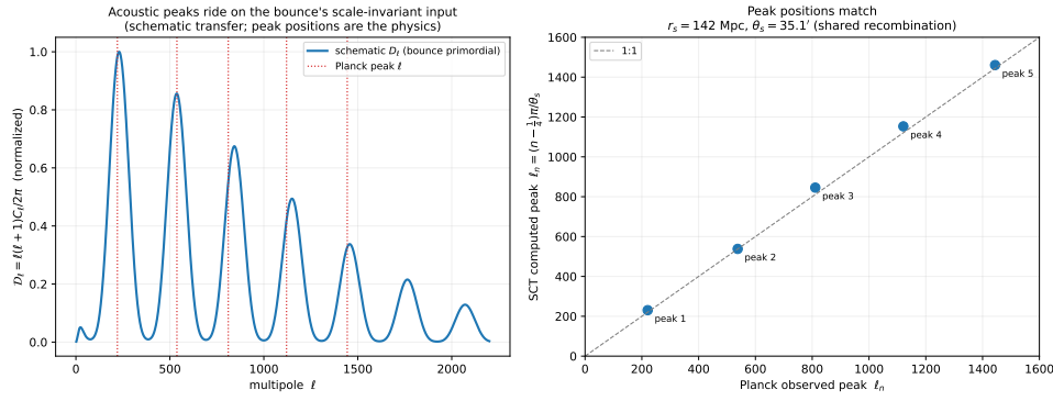
Figure 8.4: The acoustic peaks. The bounce’s scale-invariant primordial input, carried through the standard post-bounce plasma, yields a sound horizon r_s \simeq 142 \text{ Mpc} and a peak series matching the observed Planck multipoles to a few percent. The peak heights await a full Boltzmann computation. Reproducible as figures/scripts/ch09_acoustic.py .
