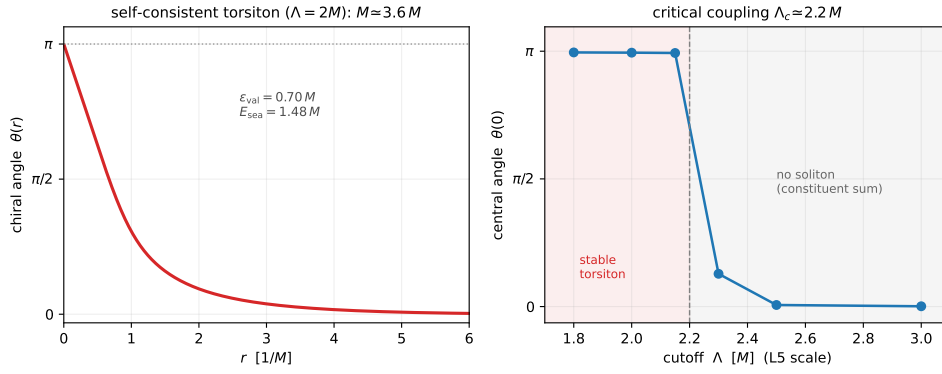
Figure C.1: The torsiton as a self-consistent chiral soliton. Left : the chiral angle \theta(r) of the B=1 torsiton, solved fully self-consistently (the profile determined by the quark source, not assumed) in the Kahana–Ripka chiral-quark-soliton model at strong coupling \Lambda = 2M —a clean hedgehog winding \theta(0) = \pi \rightarrow 0 over \sim 2/M , with mass M_{\text{torsiton}} = N_c \epsilon_{\text{val}} + E_{\text{sea}} \simeq 3.6M \simeq N_c M . Right : the converged central angle \theta(0) versus the cutoff \Lambda (the L5 scale), showing the critical coupling \Lambda_c \simeq 2.2M : below it a stable torsiton forms ( \theta(0) = \pi ); above it the soliton dissolves to the vacuum and the B=1 sector is the unbound constituent sum. Reproduced by figures/scripts/appC_torsiton_profile.py .
