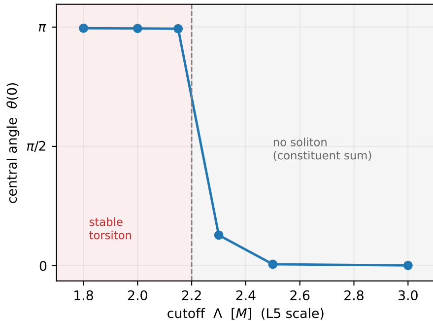
critical coupling \Lambda_c \approx 2.2 M
