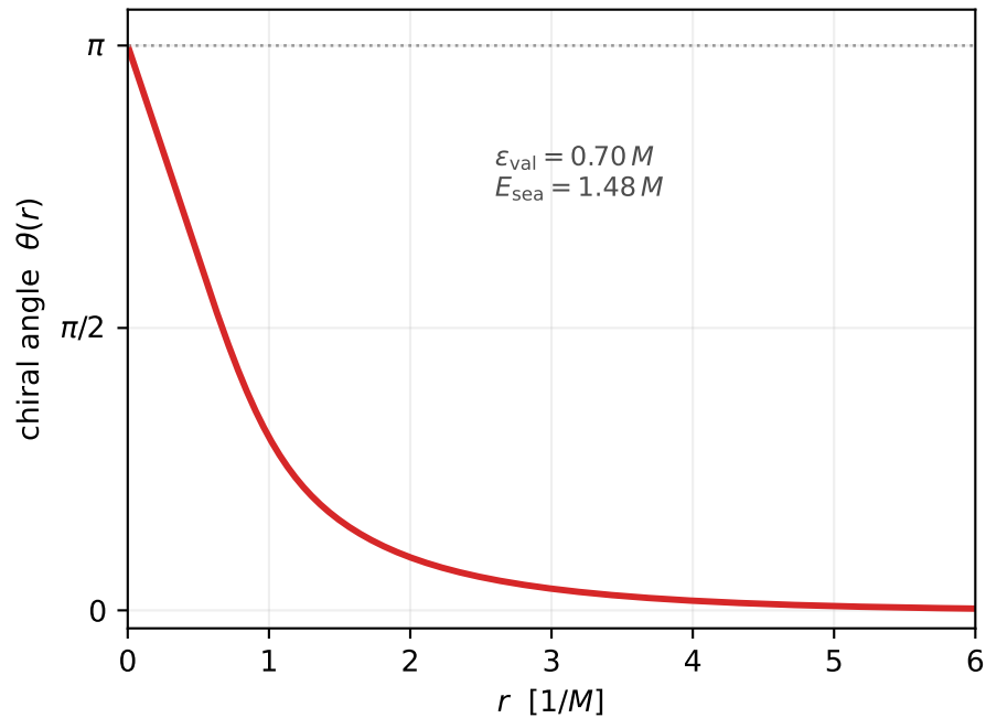
self-consistent torsiton ( \Lambda = 2M ): M \approx 3.6 M
