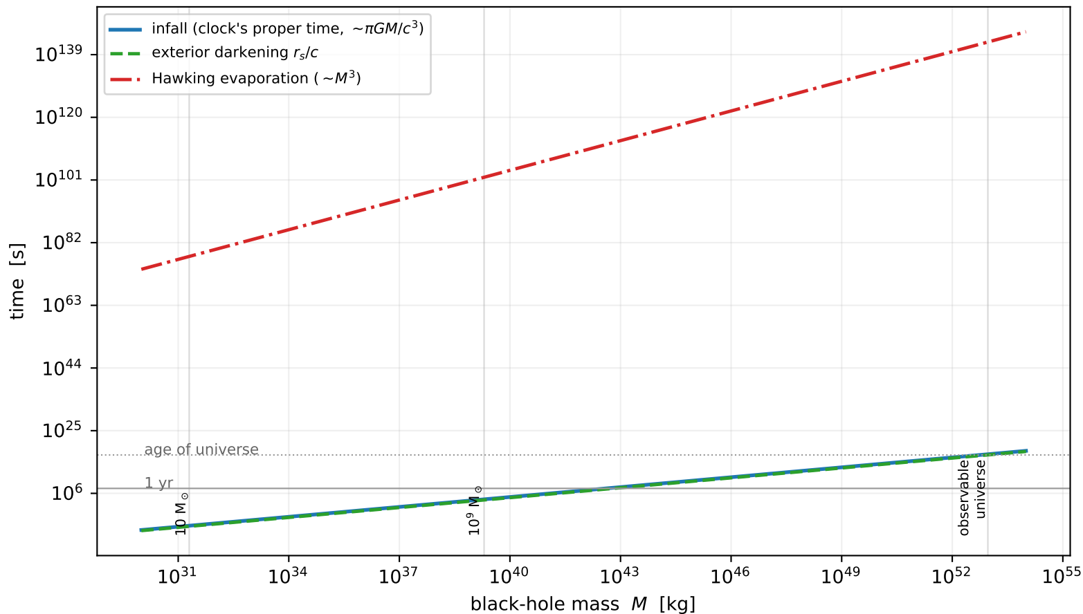
A clock's journey: proper infall ( \sim M ) vs Hawking return ( \sim M^3 )
