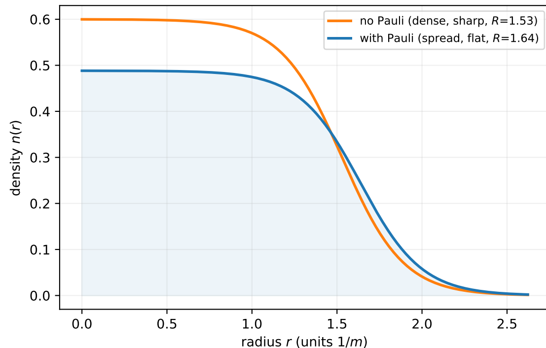
The drop: Pauli makes it larger and flatter (box-like interior = 'walking' = helps S )
