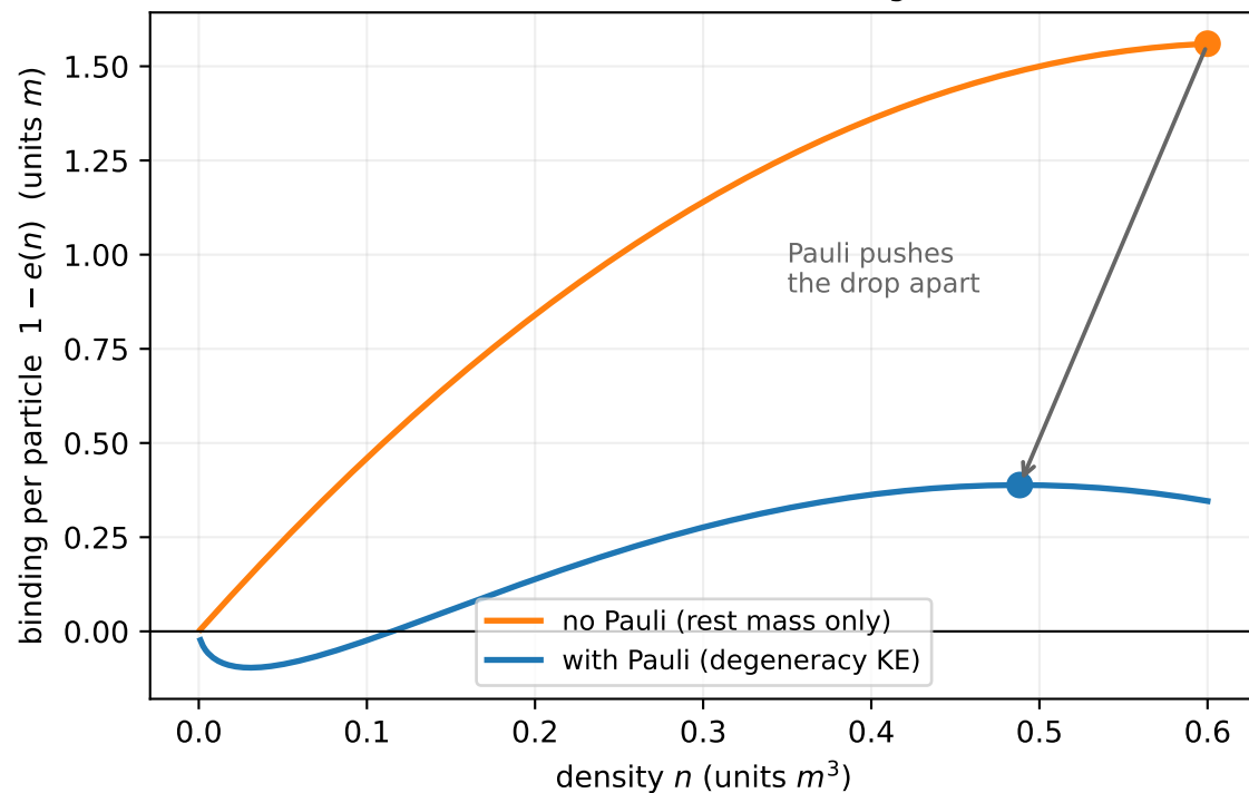
Degeneracy lowers the saturation density and shallows the binding
