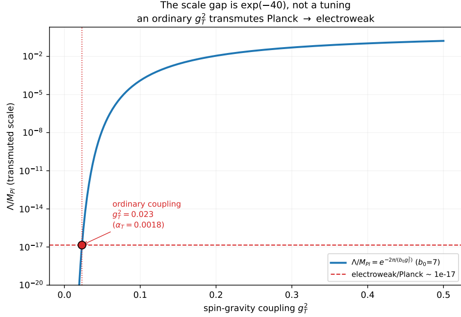
Figure 6.1: The infrared scale by dimensional transmutation, Eq. (6.1). The electroweak-to-Planck ratio is e^{-40} \approx 10^{-17} , the exponential of an ordinary coupling g^2 \sim 0.02 (weaker than electromagnetism). Fixing the scale here, once, lets the rest of Part II work in physical units—the same step \Lambda_{\text{CDM}} makes for \Lambda_{\text{QCD}} .
