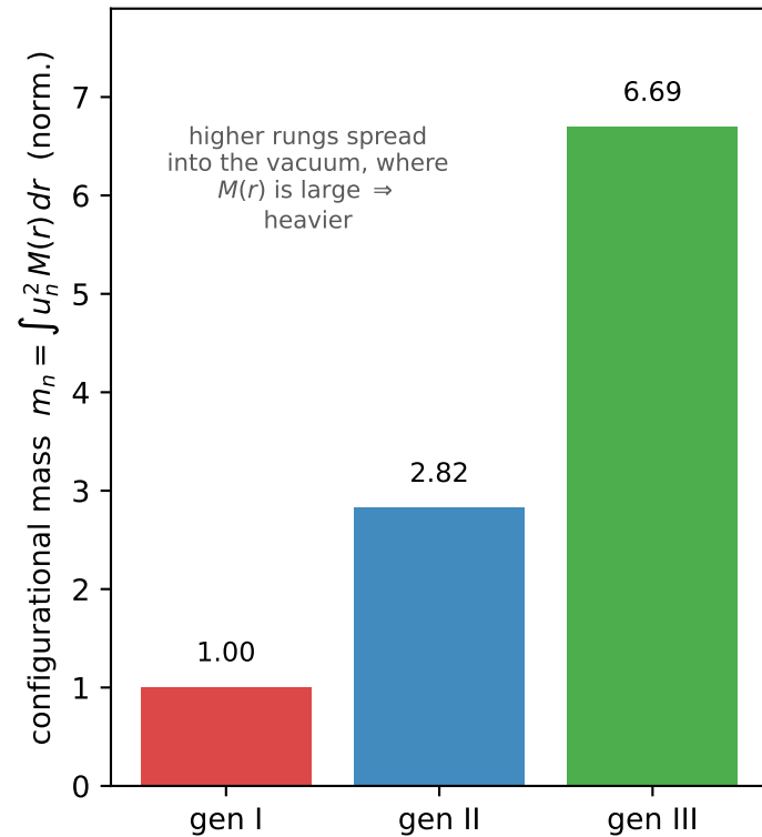
mass = overlap with M(r)
