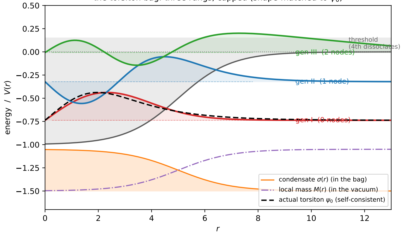
the torsiton bag: three rungs, capped (shape-matched to \psi_0 )
