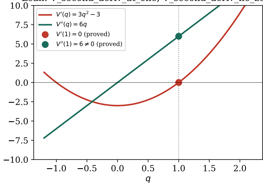
Whitney A_1 Conditions Verified Lean: V\_second\_deriv\_at\_one, V\_second\_deriv\_ne\_zero
