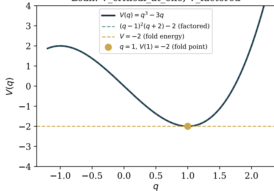
Whitney A_1 Fold Potential Lean: V\_critical\_at\_one, V\_factored
