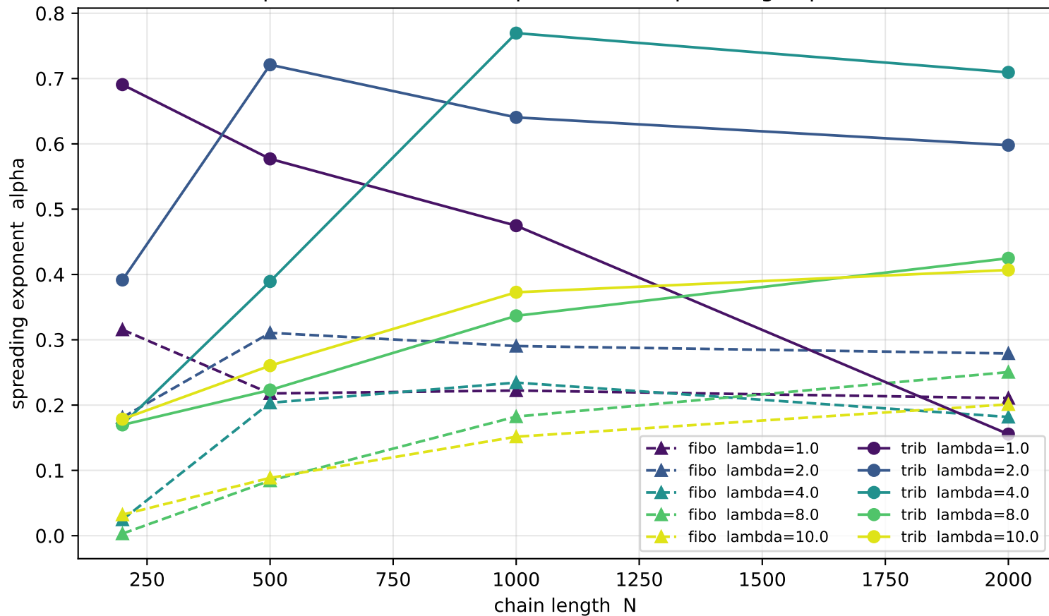
\alpha(N) -- finite-size dependence of spreading exponent
