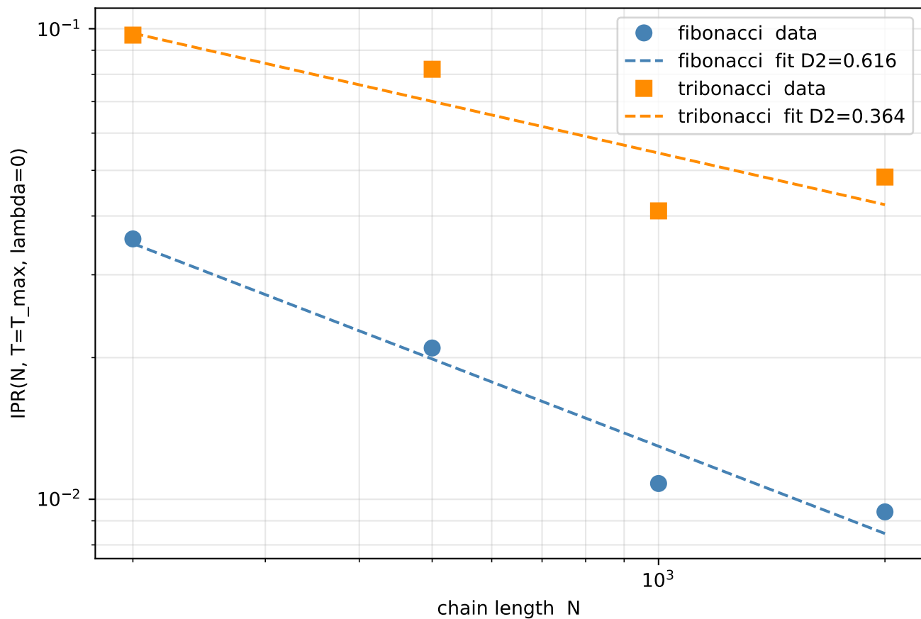
D2 multifractal dimension (linear limit, lambda=0)
