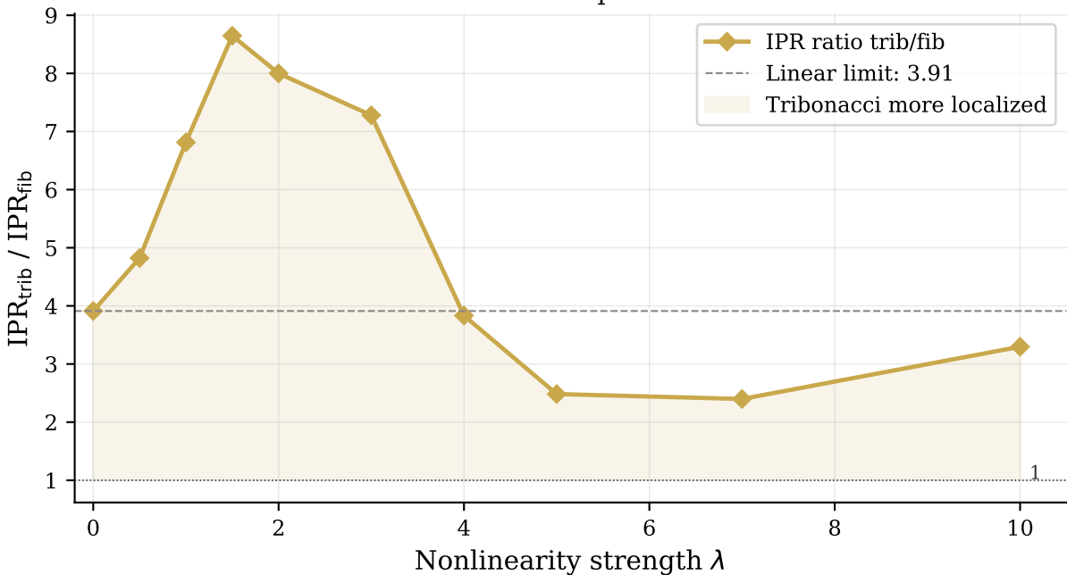
Localization advantage of tribonacci chain under nonlinear perturbation
