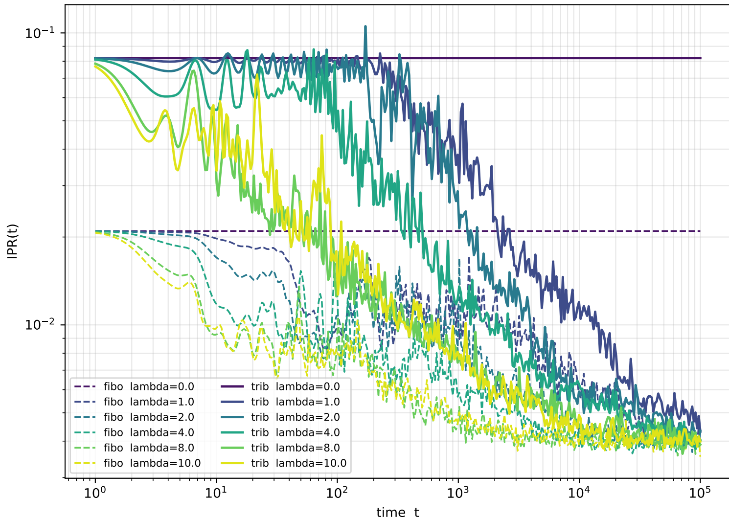
Long-time IPR on Fibonacci (dashed) and Tribonacci (solid) chains
