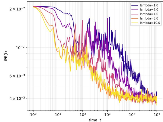
fibonacci (dotted = late-time t^{-\alpha} fit)
