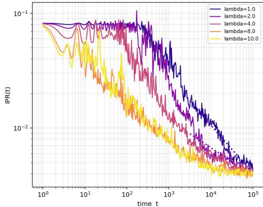
tribonacci (dotted = late-time t^{-\alpha} fit)
