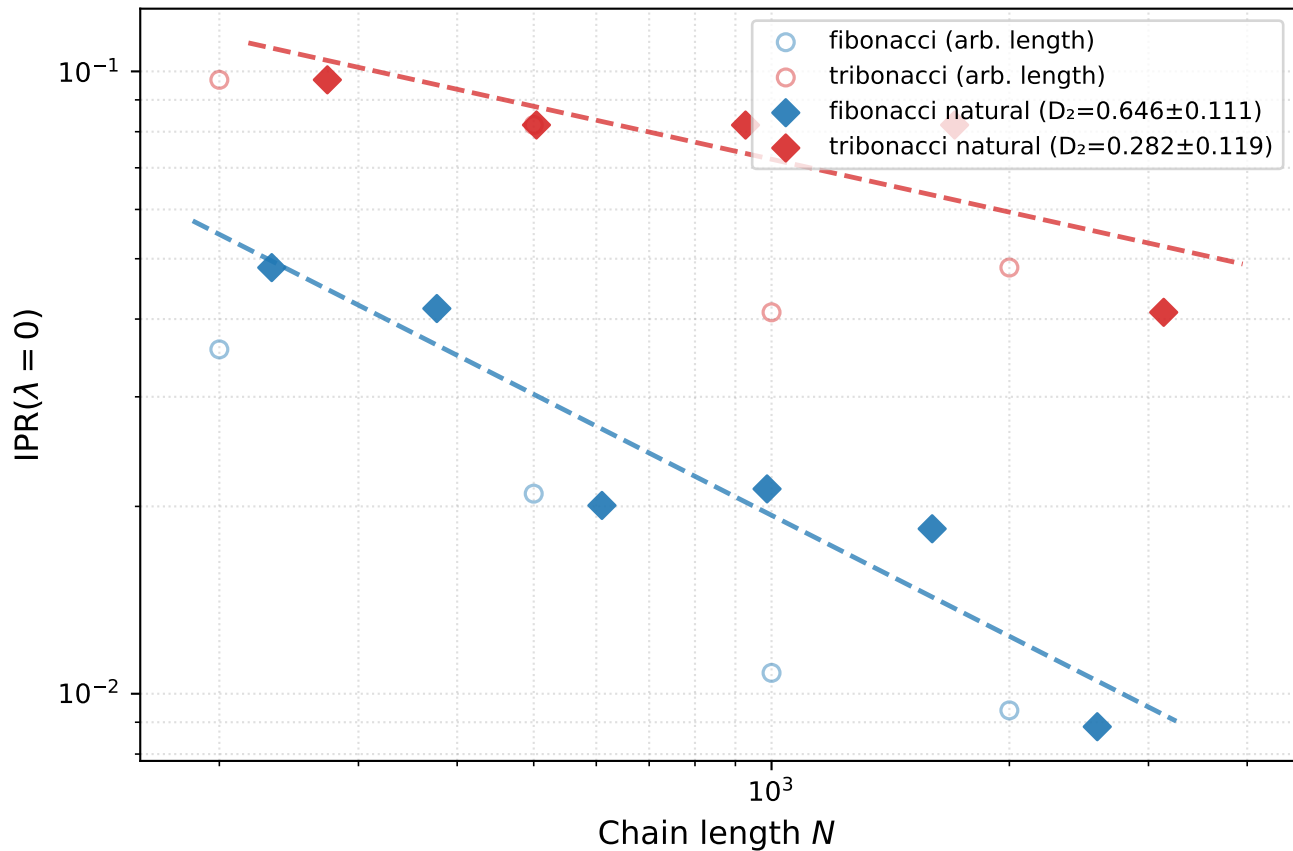
Fig A — IPR vs N at \lambda = 0 : natural vs arbitrary chain lengths
