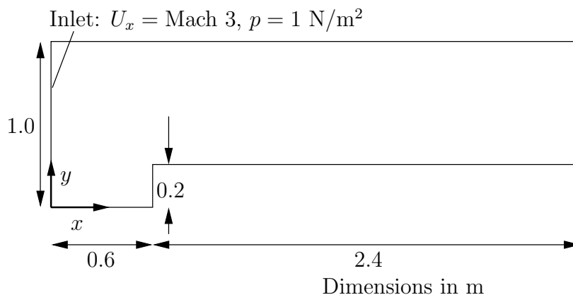
Figure 3.4: Geometry of the forward step geometry
