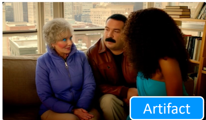
MultiShot Master14B
