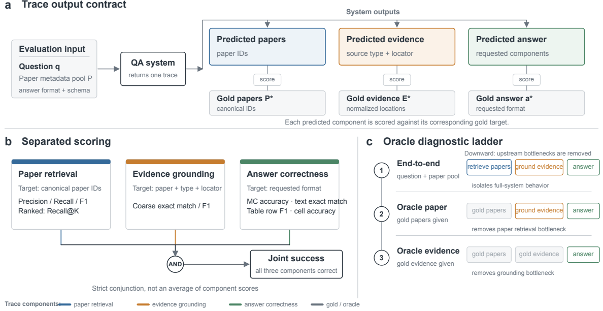
Figure 3: Detailed LitTraceQA evaluation protocol. Systems return papers, evidence locations, and answers. Component metrics diagnose each stage; strict joint success requires all stages to be correct; oracle settings remove upstream bottlenecks without implying additional baseline results.
