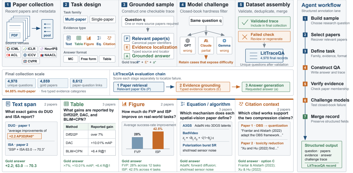
Figure 1: LITTRACEQA connects scientific-paper collection, grounded question construction, closed-book challenge, and validation. Each retained record links a question to one or more gold papers, typed evidence, and a checkable answer; evaluation follows the paper-retrieval, evidence-grounding, and answer-generation trace.
