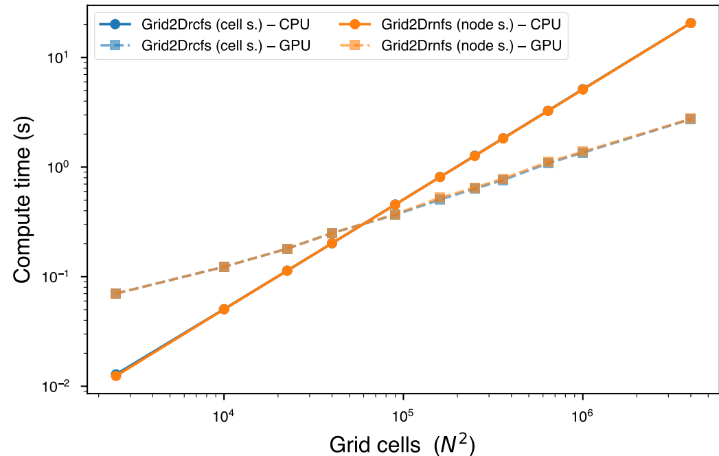
Compute time vs grid size
