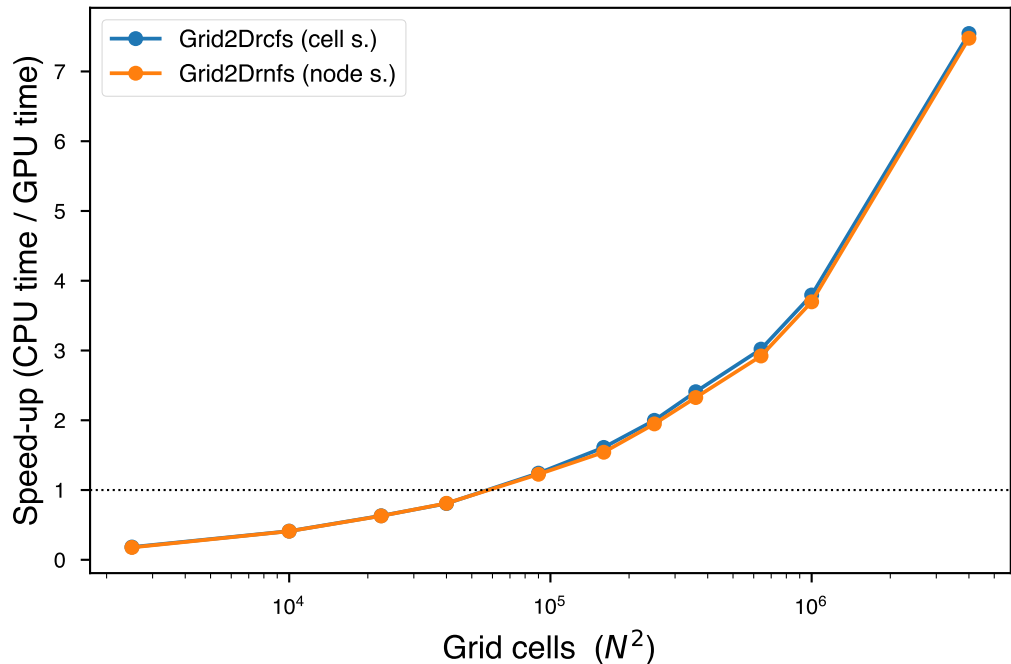
GPU speed-up vs grid size
