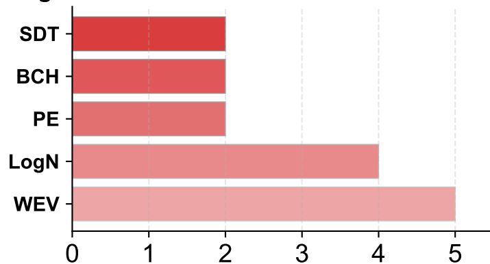
b) Logits-based
