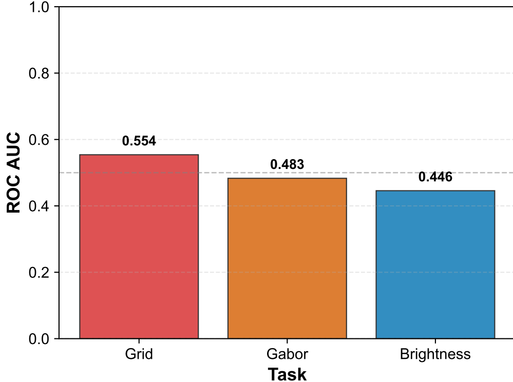
B) Area Under ROC Curve
