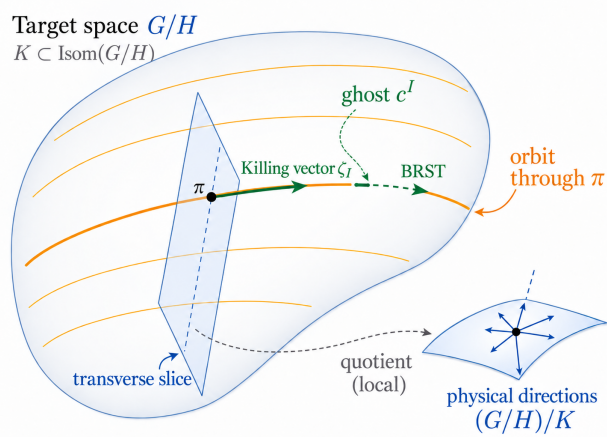
Figure 1: Geometric interpretation of Killing directions and BRST reduction for the NL \sigma M and spaces generated after SSB. The Killing vectors ( \zeta_I ) yields the infinitesimal action of the symmetry group K on the target space (G/H) and are tangent to the symmetry orbits. After gauge fixing procedure, the BRST transformation follows these same symmetry directions, with the ghost fields ( c^I ) providing their Grassmann-odd extension. A local transverse plane on \pi represents the separation between gauge directions and locally independent configurations while the reduced space illustrates the geometrical counterpart of eliminating the gauge redundancies with the BRST-cohomology with the BRST-cohomology. The graphical representation for this geometric interpretation was developed with the assistance of generative AI tools (GPT 5.6-model).
