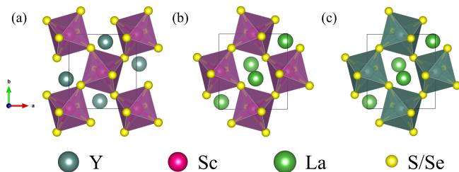
FIG. 1. Crystal structures of rare-earth chalcogenide perovskites (a) YScX_3 , (b) LaScX_3 , and (c) LaYX_3 , respectively, where X = S, Se .
