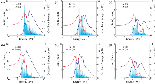
FIG. 4. Spatially averaged real [\text{Re}(\epsilon)] and imaginary part [\text{Im}(\epsilon)] of the electronic dielectric function for rare-earth chalcogenide perovskites (a) YScS 3 , (b) YScSe 3 , (c) LaScS 3 , (d) LaScSe 3 , (e) LaYS 3 , and (f) LaYSe 3 , respectively, calculated using the BSE@G 0 W 0 @PBE method. Peaks with cyan color represent the oscillator strength.
