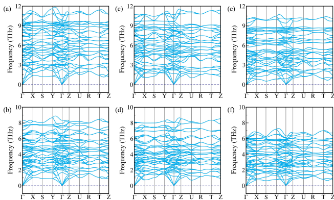
FIG. 2. Phonon dispersion curves of the rare-earth chalcogenide perovskites (a) \text{YScS}_3 , (b) \text{YScSe}_3 , (c) \text{LaScS}_3 , (d) \text{LaScSe}_3 , (e) \text{LaYS}_3 , and (f) \text{LaYSe}_3 , computed using the DFPT method based on PBEsol-relaxed structures.
