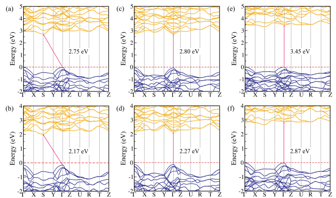
FIG. 3. Electronic band structures of the rare-earth chalcogenide perovskites (a) \text{YScS}_3 , (b) \text{YScSe}_3 , (c) \text{LaScS}_3 , (d) \text{LaScSe}_3 , (e) \text{LaYS}_3 , and (f) \text{LaYSe}_3 , calculated using the HSE06 xc functional. The Fermi level is set to be zero and marked by the dashed line.
