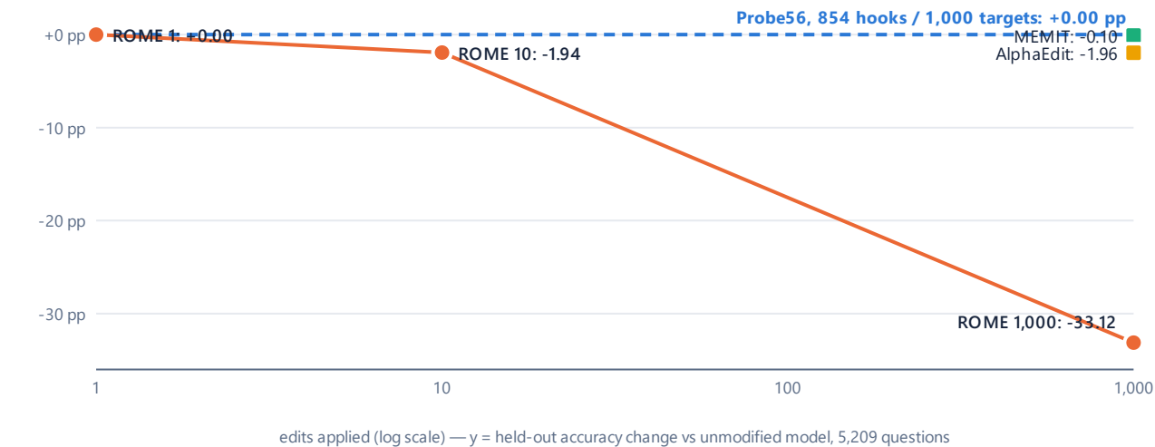
Figure 2 — ROME collateral vs edit count
