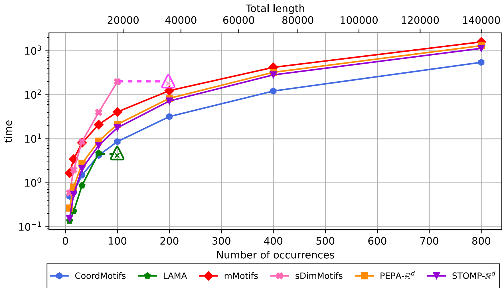
(b) Time Series length
