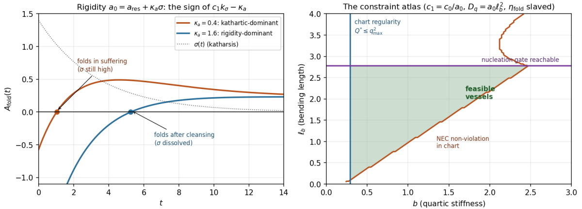
Figure 14.1: Left: the rigidity postulate's dichotomy — A_{\text{fold}}(t) along the same kathartic trajectory ( \sigma(t) dotted) for a kathartic-dominant vessel ( \kappa_a = 0.4 : folds at t = 1.0 , in suffering) and a rigidity-dominant one ( \kappa_a = 1.6 : folds at t = 5.3 , after cleansing); onset markers on the zero line. Right: the constraint atlas in the (b, \ell_b) plane with c_1 = c_0/a_0 , D_q = a_0\ell_b^2 , \eta_{\text{fold}} slaved: chart regularity (vertical), nucleation reachability (horizontal), NEC non-violation (curve); the shaded set is the space of feasible vessels. Illustrative statistics \bar{\lambda} = 1.5 , \sup \dot{\lambda}^0 = 2 , q_{\text{max}}^2 = 1.2 , c_w = 0.6 .
