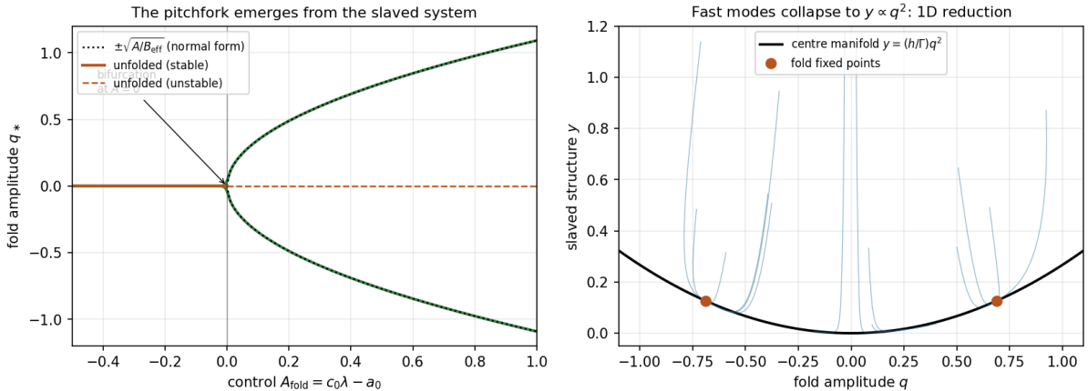
Figure 6.1: Left: the bifurcation diagram of the full two-mode slaved system (green) against the reduced normal form \pm \sqrt{A_{\text{fold}}/B_{\text{eff}}} (dotted) — the unfolded state (orange) loses stability at A_{\text{fold}} = 0 and the symmetric pair of folded states emerges: a pitchfork, derived not posited. Right: the centre-manifold geometry — trajectories of the fast structural mode y collapse onto y = (h/\Gamma)q_{\text{fold}}^2 (black), reducing the dynamics to one dimension; fold fixed points marked. Parameters b_3 = 1 , g = 0.6 , \Gamma = 3 , h = 0.8 , giving B_{\text{eff}} = 0.84 .
