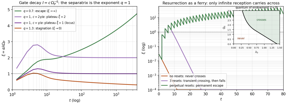
Figure 22.1: Left: the gate-decay trichotomy for I_{\text{gate}} = c\Omega_P^{-q} — escape at q = 0.7 ; tunable plateaus \bar{\xi} = \alpha c/\gamma at q = 1 (shown: \bar{\xi} = 1 , the locus, and \bar{\xi} = 2 ); stagnation at q = 1.3 . The separatrix is the exponent. Right: the resurrection ferry for the closed vessel (log scale): no resets never cross; three resets cross transiently ( \max \xi = 3.0 ) and fall back into dissolution; perpetual resets ( g_0 = 0.6 , m_0 = 0.5 , \Delta = 2 ) escape permanently with converging budget. Inset: the quantum-of-endowment boundary in the (\lambda_0, \Omega_P(0)) plane — the hyperbola \xi_0 = 1 for small \lambda_0 , the line \sqrt{\gamma}(\Omega_P(0) + \beta) = 2 beyond. Parameters \alpha = 1 , \gamma = 0.5 , illustrative.
