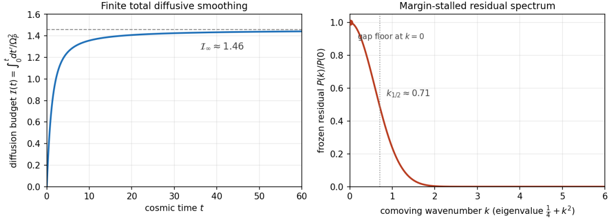
Figure 8.1: Left: the diffusive smoothing budget \mathcal{I}(t) = \int_0^t dt'/\Omega_P^2 saturates to a finite \mathcal{I}_\infty (illustrative background \lambda_0 = 0.4 \rightarrow \lambda_\infty = 1 , \Omega_P(0) = 1 ). Right: the margin-stalled frozen residual spectrum P(k)/P(0) (with D = 0.5 ): the hyperbolic gap leaves a k = 0 floor while small scales are erased, defining a structure scale k_{1/2} \approx 0.71 . Parameters illustrative.
