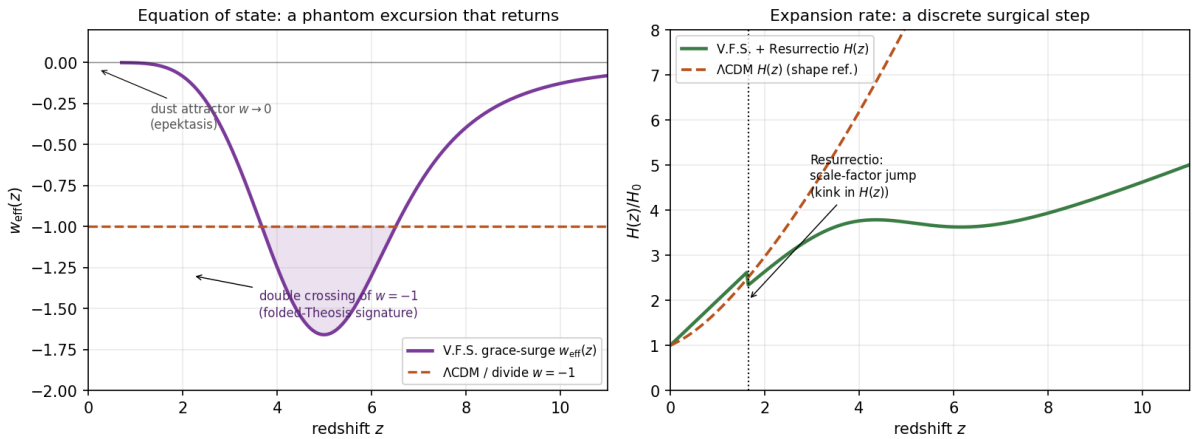
Figure 26.1: Left: w_{\text{eff}}(z) for a grace-surge trajectory (purple) against the \Lambda CDM/divide line w = -1 (dashed). The curve coasts toward dust ( w_{\text{eff}} \rightarrow 0 ) at low z , and during the surge dips below -1 and returns — a double crossing (shaded), the folded-Theosis signature, impossible for smooth single-field quintessence. Right: H(z)/H_0 for a trajectory with a Resurrectio reset (green) against a \Lambda CDM shape reference (dashed): the reset prints a kink at z \approx 1.65 and a non-monotone, displaced history — a discrete surgical step no smooth dark energy contains. Exact reconstructions along admissible ( I_{\text{gate}} \geq 0 ) trajectories; 2+1, illustrative parameters.
