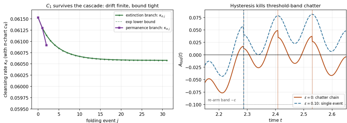
Figure 7.1: Left: survival of the cleansing rate \kappa_{\sigma,j} (computed with the \pi -chart c_\Psi ) along both terminal branches of the forced-folding cascade; the exponential lower bound of Proposition 7.2 overlays the actual sequence — tight to four digits. The drift is finite because the metabolic budget is. Right: the Zeno mechanism and its cure. With \varepsilon = 0 (solid) the update's downward A_{\text{fold}} -jump re-arms the event machine between fast crests of the quasi-periodic resistance wave, producing a chatter chain of three events at gaps \approx 0.12 ; with \varepsilon = 0.10 (dashed) the band swallows the re-arming and a single event per slow peak remains — the minimal dwell grows by a factor 18.5. Parameters illustrative.
