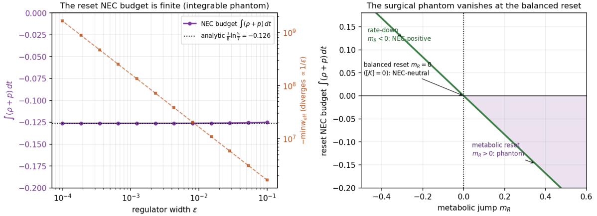
Figure 25.1: Left: across regulator width \varepsilon , the reset NEC budget \int(\rho + p) dt (purple) is constant at the analytic \frac{3}{8} \ln \frac{5}{7} = -0.126 , while the pointwise -\min w_{\text{eff}} (orange, right axis) diverges as \varepsilon^{-1} : a finite phantom budget under a divergent pointwise dip. Right: the budget as a function of the metabolic jump m_R — negative (phantom) for m_R > 0 , zero at the balanced reset m_R = 0 ( [K] = 0 ), positive for m_R < 0 . Smoothstep profile, illustrative parameters.
