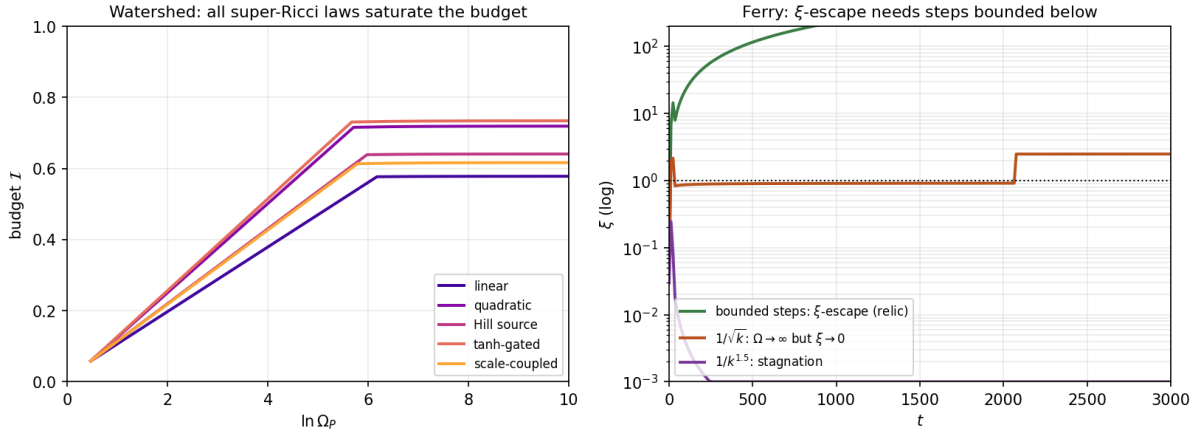
Figure 17.1: Left: the watershed under closure deformation — five inequivalent Sophia laws, all sustained, all saturating the budget \mathcal{I} at a finite value (super-Ricci relic class); the classification is premise-independent. Right: the ferry distinction — bounded reset steps give genuine \xi -escape (relic with vitality); 1/\sqrt{k} steps inflate the Brim ( \Omega_P \rightarrow \infty ) but let \xi \rightarrow 0 (relic without vitality); 1/k^{1.5} steps stagnate. \Omega_P -escape and \xi -escape are distinct, and only the latter is the ferry's claim.
