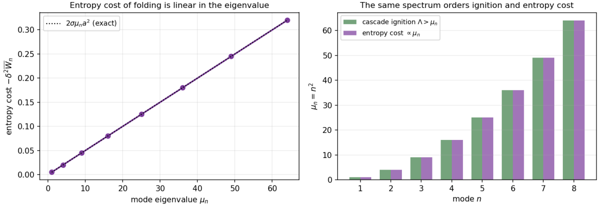
Figure 21.1: Left: the entropy cost -\delta^2 \overline{W}_+^{(n)} of folding mode n , exactly 2\sigma\mu_n a_n^2 (dotted), linear in the eigenvalue. Right: the same spectrum \mu_n = n^2 orders both the cascade ignition ladder ( \Lambda > \mu_n , the mode-cascade chapter) and the entropy cost — the higher the rung, the dearer the fold. Ring proxy, a = 0.05 .
