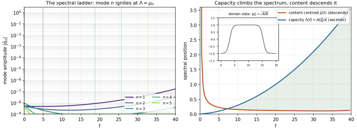
Figure 16.1: Left: the spectral ladder on the ring proxy — mode amplitudes |\hat{q}_n| against time, each turning from decay to growth at its own vertical \Lambda(t) = \mu_n (dotted), in strict spectral order n = 1, 2, \dots . Right: the scissoring of structure formation — the capacity \Lambda(t) (blue, ascending) against the content centroid \bar{\mu}(t) (orange, descending); the shaded gap is the band of ignited-but-not-yet-coarsened modes. Inset: the developed multi-mode domain state, whose interior saturates to \sqrt{A_{\text{fold}}/B_{\text{fold}}} regardless of mode count. Ring proxy, \hat{\kappa} = 0.5 .
