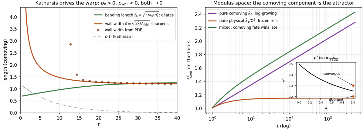
Figure 15.1: Left: the two channel lengths along one kathartic trajectory ( \sigma(t) dotted): the bending length \ell_b dilates while the wall width \delta_{\text{wall}} sharpens (full PDE measurements as points; the early outlier is the adiabatic lag near threshold), both settling to comoving constants as \sigma dissolves. Right: modulus space on the resonance locus — pure comoving modulus gives the log-growing coarsening, a pure \Omega_P^{-2} modulus freezes a relic, and any mixture rejoins the comoving fate: the comoving component is the attractor. Inset: the generalised watershed p^*(w) = 1/(2 + 2w) with the verified convergence/divergence pair at w = 1 .
