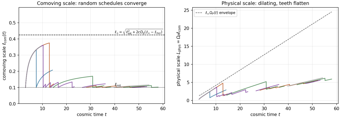
Figure 12.1: Reduced recursion over five random reset schedules (non-Zeno spacing; rescale/trigger/quench with probabilities 0.7/0.15/0.15; illustrative 2cD_q = 0.5 , \ell_{\text{init}} = 0.1 , \mathcal{I}_\infty \approx 1.46 ). Left: the comoving scale \ell_{\text{com}}(t) — early arcs coarsen substantially toward \ell_\infty , but as the budget depletes the teeth flatten and every schedule is pinned near \ell_{\text{init}} at late times. Right: the physical scale L_{\text{phys}} = \Omega_P \ell_{\text{com}} dilates along the \ell_\infty \Omega_P(t) envelope; gaps are quench intervals (network dissolved). Comoving teeth flatten; physical scale keeps dilating \propto \Omega_P \propto t .
