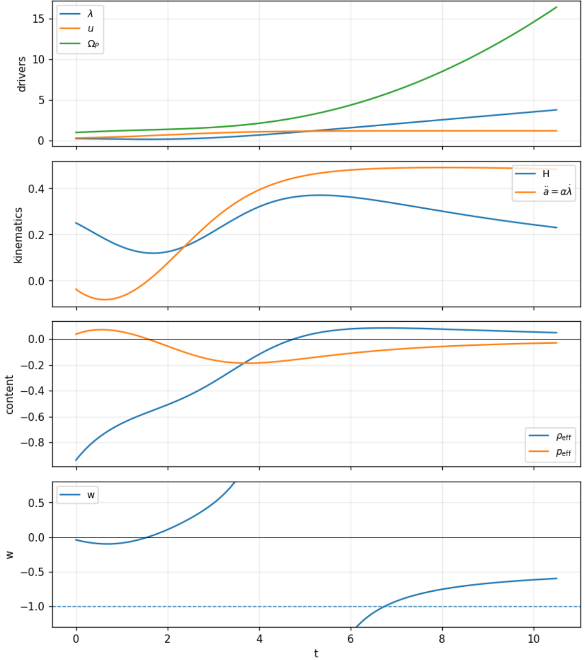
Figure 1: Open-Gate Vessel cosmology along a Sophia trajectory. From top: drivers \lambda, u, \Omega_P ; Hubble rate and acceleration \ddot{a} = \alpha \dot{\lambda} ; effective density and pressure; the equation of state w(t) with its pole at the Milne crossing \rho_{\text{eff}} = 0 . In the integrated folding interpretation, this background curve is moderated by the positive contribution \Delta q_{\text{dec}} = (\eta \Omega_P / \alpha \lambda) Q_{\text{fold}} . Shading marks the decelerating struggle, the accelerating Theosis — which in 2+1 is exactly the SEC-violation region p_{\text{eff}} < 0 — and the NEC-violation band.
