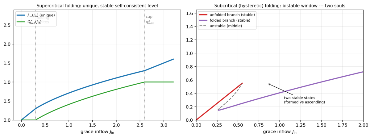
Figure 12: The self-consistent folded-ascent level. Left: supercritical folding — a single-valued \lambda_\infty(J_{in}) and Q^*(J_{in}) , folding igniting at J_{in} = \gamma a_0/c_0 and saturating at the cap q_{max}^2 ; the level is unique and stable. Right: subcritical (hysteretic) folding — the unfolded and folded branches overlap over a J_{in} -window where both are stable (unstable middle dashed): two coexisting souls, formed versus ascending. On every branch \lambda_\infty > 0 : the ascent is moderated, never abolished.
