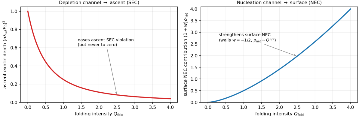
Figure 13: One Q_{\text{fold}} , two sectors. Left: the depletion channel lowers the ascent SEC exotic depth (\alpha\lambda_\infty/E_0)^2 — easing the violation, never to zero. Right: the nucleation channel builds the wall network ( \rho_{\text{net}} \sim Q_{\text{fold}}^{3/2} , walls w = -\frac{1}{2} ), whose NEC contribution (1 + w)\rho_{\text{net}} grows with folding — strengthening the surface NEC. The same folding intensity drives both, with opposite sign on the two sectors.
