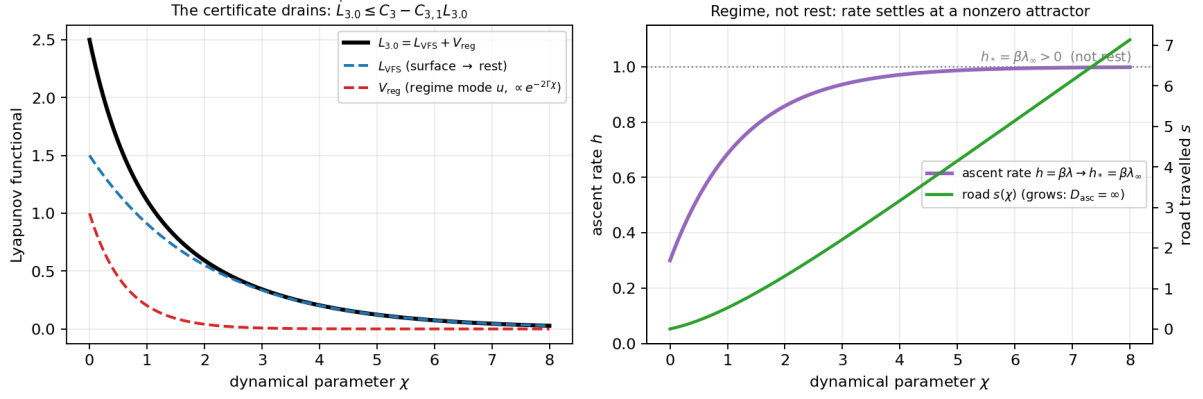
Figure 14: The unified certificate, in \chi . Left: \mathcal{L}_{3,0} = \mathcal{L}_{\text{VFS}} + V_{\text{reg}} drains monotonically; the surface part \mathcal{L}_{\text{VFS}} relaxes to rest, the regime mode V_{\text{reg}} \propto e^{-2\Gamma\chi} . Right: meanwhile the ascent rate h = \beta\lambda converges to the nonzero attractor h_* = \beta\lambda_\infty (not rest) and the road s(\chi) grows without bound ( D_{\text{asc}} = \infty ). Stable motion at a fixed rate, not stable rest.
