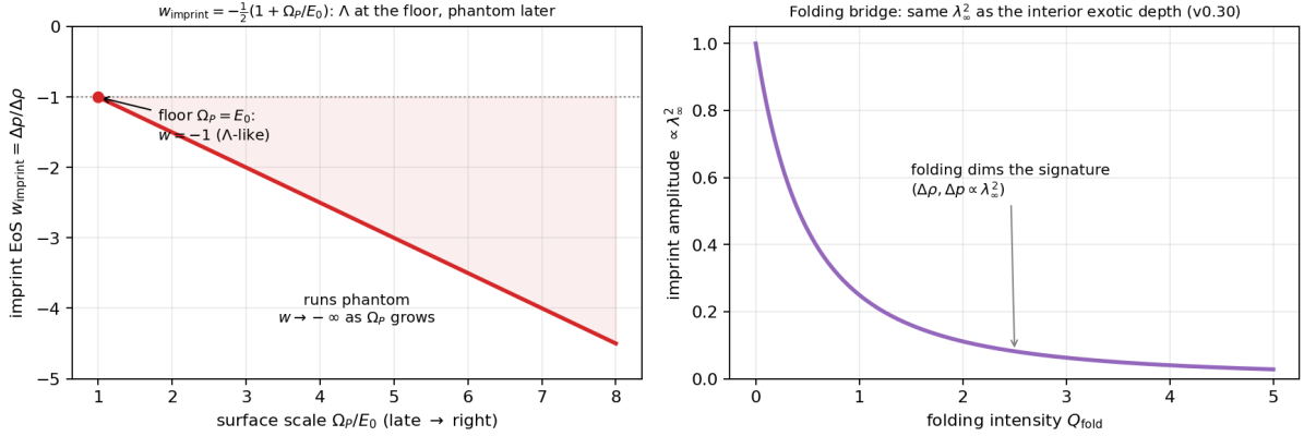
Figure 17: The completed external signature. Left: the imprint equation of state w_{\text{imprint}} = -\frac{1}{2}(1 + \Omega_P/E_0) - \Lambda -like ( w = -1 ) at the floor, running phantom as the surface scale \Omega_P/E_0 grows. Right: both imprint terms scale as \lambda_\infty^2 , so folding (which lowers \lambda_\infty , v0.30) dims the signature; this is the same \lambda_\infty^2 that sets the interior exotic depth.
