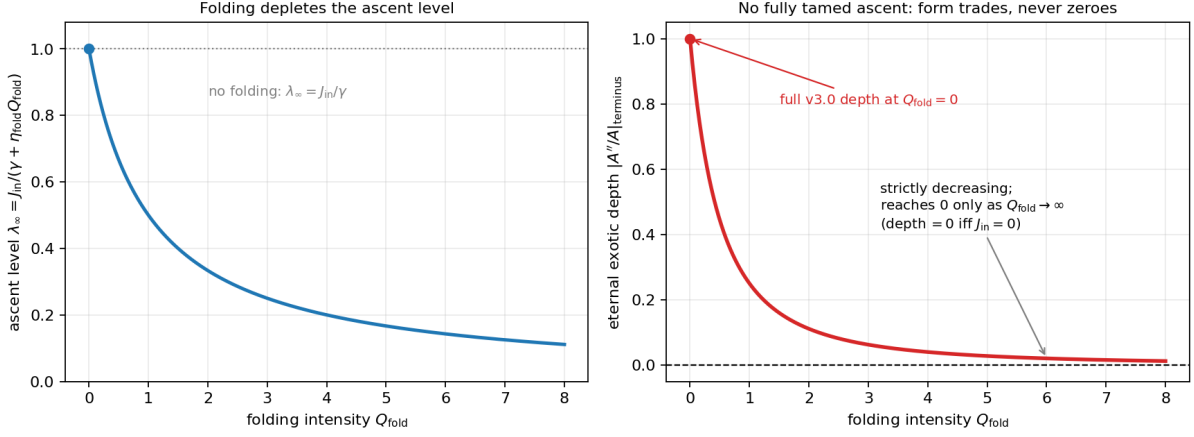
Figure 11: Folding versus the ascent. Left: the saturated ascent level \lambda_\infty = J_{\text{in}}/(\gamma + \eta_{\text{fold}}Q_{\text{fold}}) falls monotonically as folding embodies Sophia into form. Right: the eternal exotic depth \text{depth} = (\alpha\lambda_\infty/E_0)^2 decreases strictly but reaches 0 only as Q_{\text{fold}} \rightarrow \infty ; for every admissible source J_{\text{in}} > 0 it stays positive — no fully tamed ascent. Form trades against the ascent across the shared budget; it never zeroes it. Floor-normalised representative parameters.
