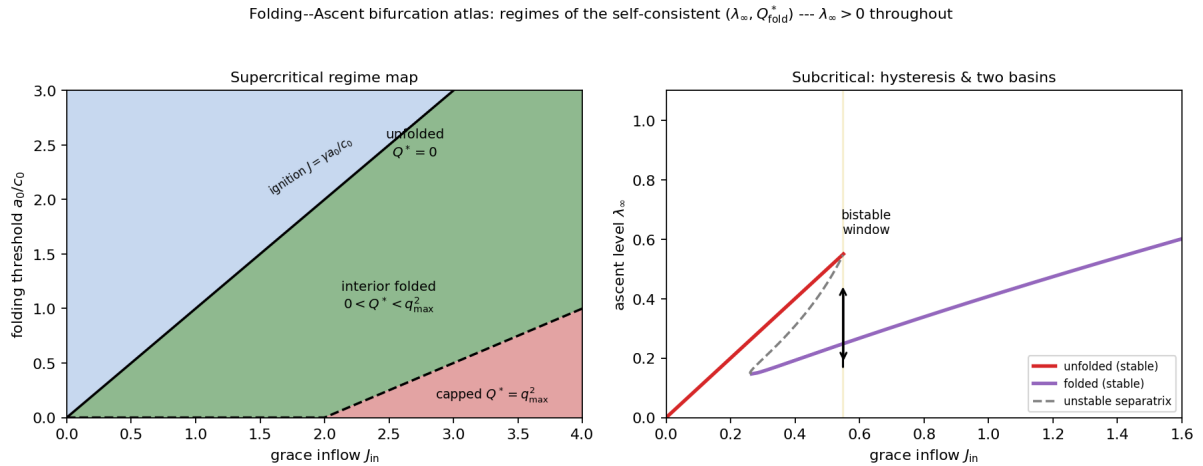
Figure 16: The Folding-Ascent bifurcation atlas. Left: supercritical regime map in the (J_{\text{in}}, a_0/c_0) plane — unfolded ( Q^* = 0 , above the ignition line J_{\text{in}} = \gamma a_0/c_0 ), interior-folded, and capped ( Q^* = q_{\text{max}}^2 ) regions. Right: the subcritical branch — a hysteresis loop over the bistable window, the unfolded and folded basins separated by the unstable separatrix (v0.38: locally, not globally, bistable). Everywhere \lambda_\infty > 0 .
