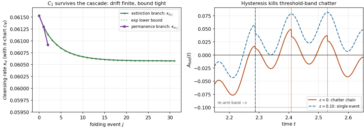
Figure 4.1: Left: survival of the cleansing rate \kappa_{\sigma,j} (computed with the \pi -chart c_\Psi ) along both terminal branches of the forced-folding cascade; the exponential lower bound of Proposition 4.2 overlays the actual sequence — tight to four digits. The drift is finite because the metabolic budget is. Right: the Zeno mechanism and its cure. With \varepsilon = 0 (solid) the update's downward A_{\text{fold}} -jump re-arms the event machine between fast crests of the quasi-periodic resistance wave, producing a chatter chain of three events at gaps \approx 0.12 ; with \varepsilon = 0.10 (dashed) the band swallows the re-arming and a single event per slow peak remains — the minimal dwell grows by a factor 18.5. Parameters illustrative.
