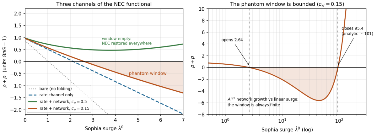
Figure 11.1: Left: the NEC functional against surge strength for the four cases (bare; rate channel only; rate+network at two network strengths), at \alpha\lambda = 1.5 , \Omega_P = 1.2 , \chi = 0.538 . The bare functional breaks at \dot{\lambda}^0 = 1.05 ; the rate channel delays this to 2.15 (the factor 1/\chi \approx 2 ) and then saturates; the strong network ( c_w = 0.5 ) keeps \mathcal{N} > 0 everywhere (empty window); the weak network ( c_w = 0.15 ) leaves a phantom window (shaded). Right: the same weak-network functional on a log axis: the window is bounded, [2.64, 95.4] , closed by the A_{\text{fold}}^{3/2} growth of the wall term; the analytic closure estimate is \sim 101 .
