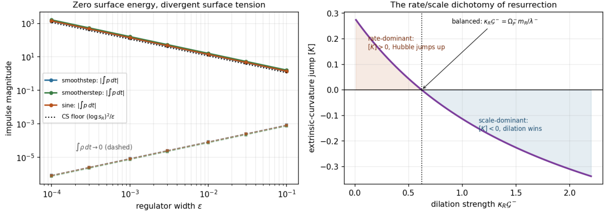
Figure 13.1: Left: regularised impulse magnitudes versus regulator width \varepsilon for three smooth step profiles (log-log). The tension impulse |\int p dt| (solid) scales exactly as \varepsilon^{-1} — profile-dependent coefficient, universal divergence — and respects the Cauchy-Schwarz floor (\log s_R)^2/\varepsilon (dotted); the energy impulse (dashed) vanishes as \varepsilon^{+1} . Right: the extrinsic-curvature jump [K] against dilation strength \kappa_R \mathcal{G}_{\text{recepta}}^- at fixed metabolism: rate-dominant ( [K] > 0 ), balanced ( \kappa_R \mathcal{G}_{\text{recepta}}^- = \Omega_P^- m_R / \lambda^- \approx 0.62 , K continuous), and scale-dominant ( [K] < 0 ) resurrections. Parameters illustrative.
