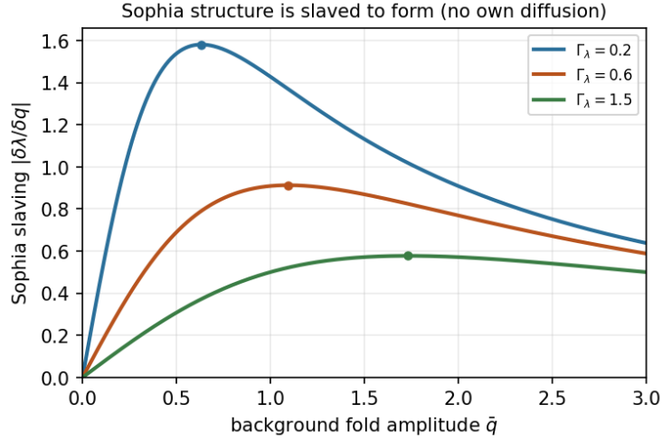
Figure 9.1: The Sophia slaving coefficient |\delta\lambda/\delta q_{\text{fold}}| = S(\bar{q}) (verified symbolically). It is bounded, vanishes at \bar{q} = 0 and at large \bar{q} , and peaks at \bar{q} = \sqrt{\Gamma_\lambda/\eta_{\text{fold}}} . Sophia inhomogeneity is sourced entirely by folding inhomogeneity; there is no independent Sophia diffusion to set. Illustrative \eta_{\text{fold}} = 0.5 , \bar{\lambda} = 1 .
