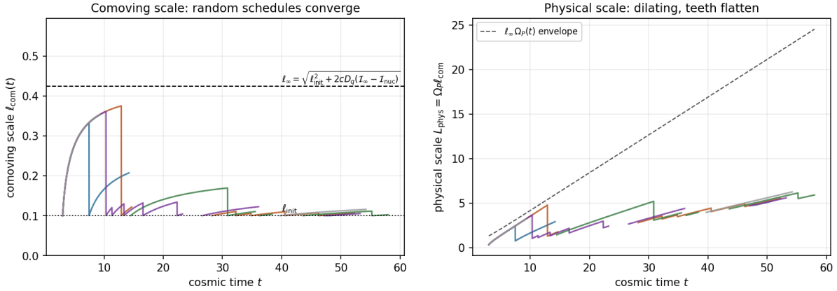
Figure 8.1: Reduced recursion over five random reset schedules (non-Zeno spacing; rescale/trigger/quench with probabilities 0.7/0.15/0.15; illustrative 2cD_q = 0.5 , \ell_{\text{init}} = 0.1 , \mathcal{I}_\infty \approx 1.46 ). Left: the comoving scale \ell_{\text{com}}(t) — early arcs coarsen substantially toward \ell_\infty , but as the budget depletes the teeth flatten and every schedule is pinned near \ell_{\text{init}} at late times. Right: the physical scale L_{\text{phys}} = \Omega_P \ell_{\text{com}} dilates along the \ell_\infty \Omega_P(t) envelope; gaps are quench intervals (network dissolved). Comoving teeth flatten; physical scale keeps dilating \propto \Omega_P \propto t .
