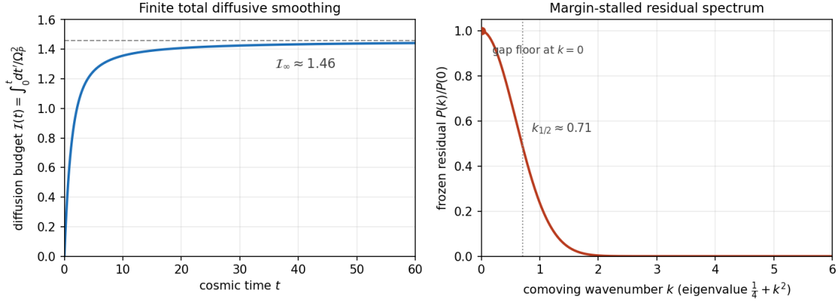
Figure 4.1: Left: the diffusive smoothing budget \mathcal{I}(t) = \int_0^t dt'/\Omega_P^2 saturates to a finite \mathcal{I}_\infty (illustrative background \lambda_0 = 0.4 \rightarrow \lambda_\infty = 1 , \Omega_P(0) = 1 ). Right: the margin-stalled frozen residual spectrum P(k)/P(0) (with D = 0.5 ): the hyperbolic gap leaves a k = 0 floor while small scales are erased, defining a structure scale k_{1/2} \approx 0.71 . Parameters illustrative.
