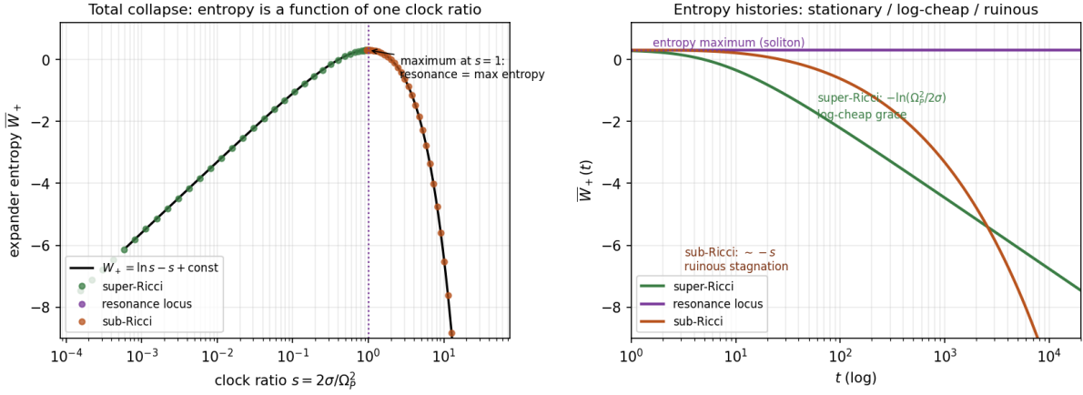
Figure 13.1: Left: total collapse — the symmetric-sector expander entropy of all three watershed trajectories (super-Ricci, locus, sub-Ricci; markers) against the clock ratio s , falling on the single universal curve \ln s - s + \text{const} (line), maximal exactly at s = 1 . Right: the entropy histories in the canonical gauge: the resonance sits at the soliton maximum; the super-Ricci flow descends logarithmically (grace is entropy-cheap); the sub-Ricci flow descends polynomially (stagnation is ruinous). Genus-2 quotient, A_h = 4\pi ; gauge \sigma_0 = \Omega_P^2(0)/2 .
