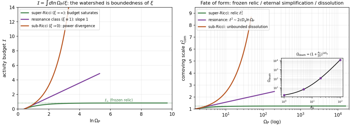
Figure 12.1: Left: the budget identity \mathcal{I} = \int d \ln \Omega_P / \xi realised on three trajectories of the same core law with different Sophia asymptotics: super-Ricci escape (budget saturates at \mathcal{I}_\infty ), the resonance locus (slope exactly 1), sub-Ricci decay (power divergence). Right: the corresponding fates of form via \ell_{\text{com}}^2 = \ell_0^2 + 2cD_q \mathcal{I} : frozen relic, eternal logarithmic simplification, unbounded dissolution. Inset: hierarchical domain death on the locus — the closed-form \Omega_P^{\text{death}}(A_0) (line) against direct integration of the Gauss-Bonnet law (points). Parameters c = 0.5 , D_q = 0.3 , \ell_0 = 1 , illustrative.
