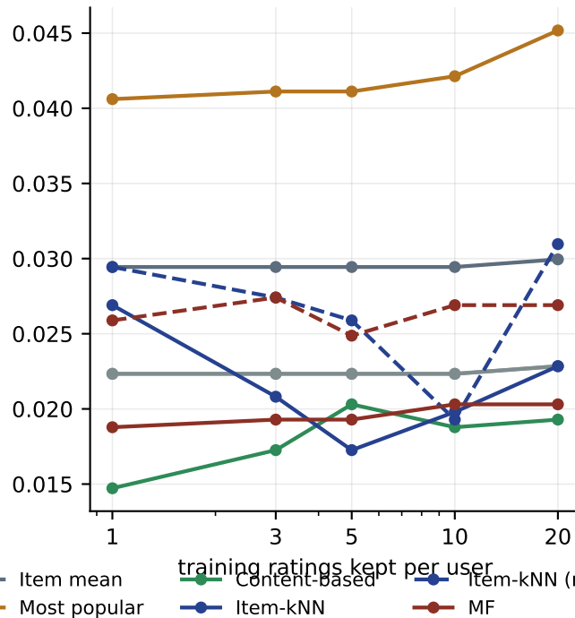
precision@10 (higher is better)
