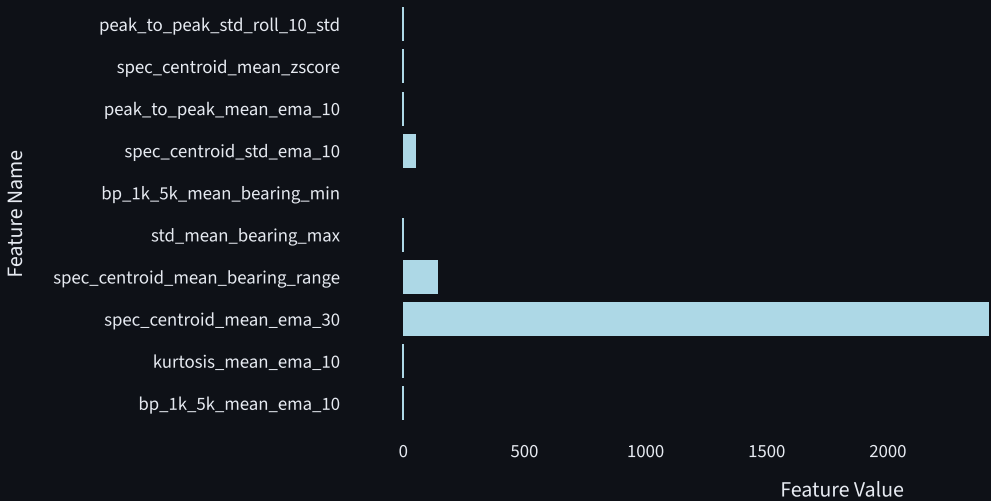
Feature Values at Current Time (Bearing 4-x)
