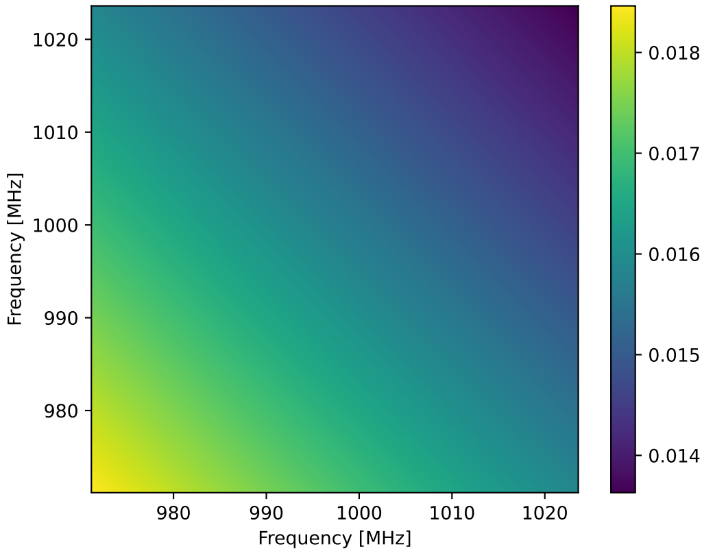
Frequency-frequency covariance
